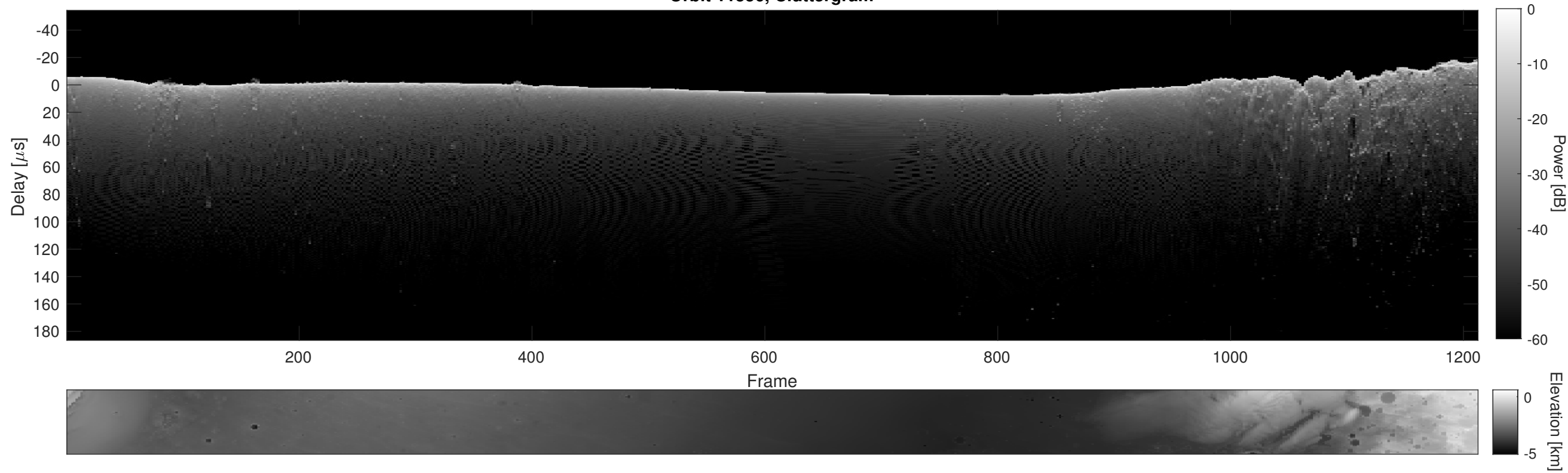
Orbit 11556, Cluttergram
