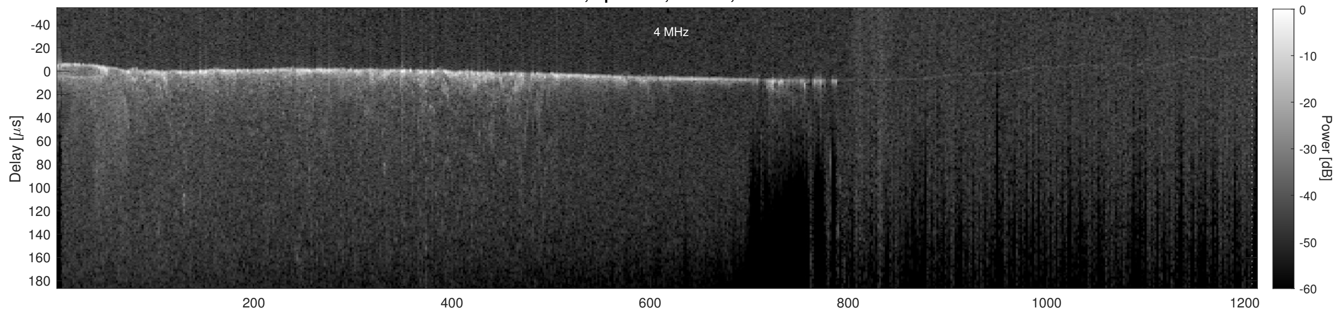
Orbit 11556, Cluttergram
