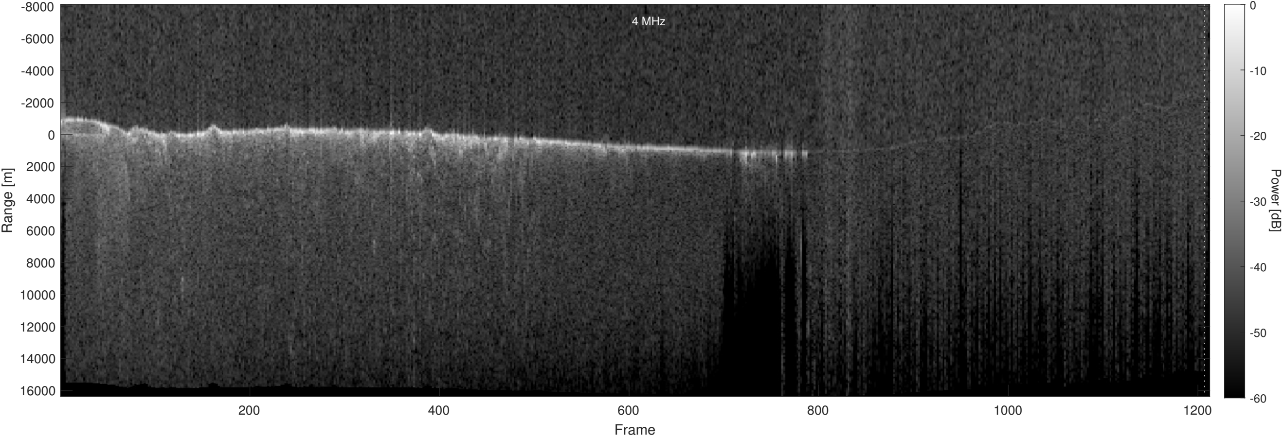
Orbit 11556, Optimized, Window, Depth-Corrected, Channel 2
