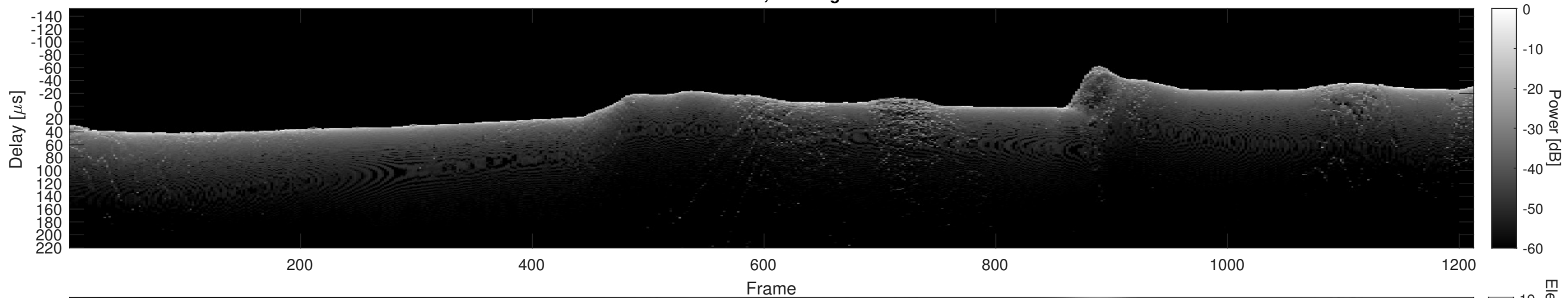
Orbit 11559, Cluttergram
