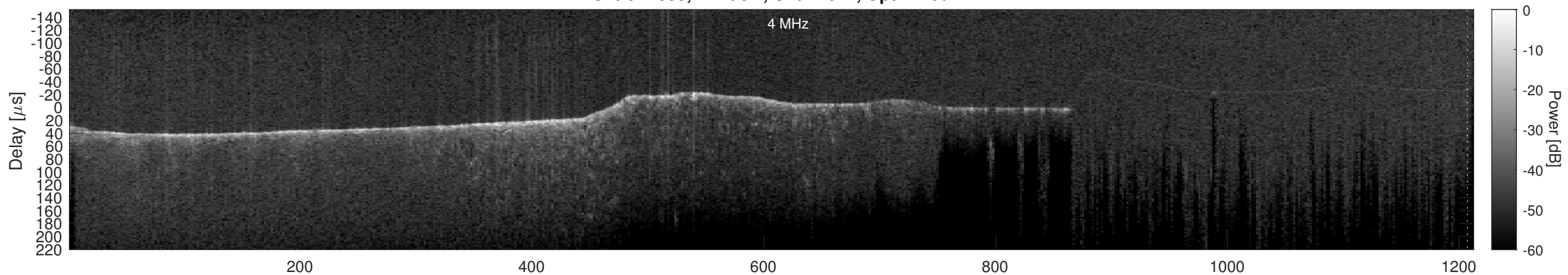
Orbit 11559, Cluttergram
