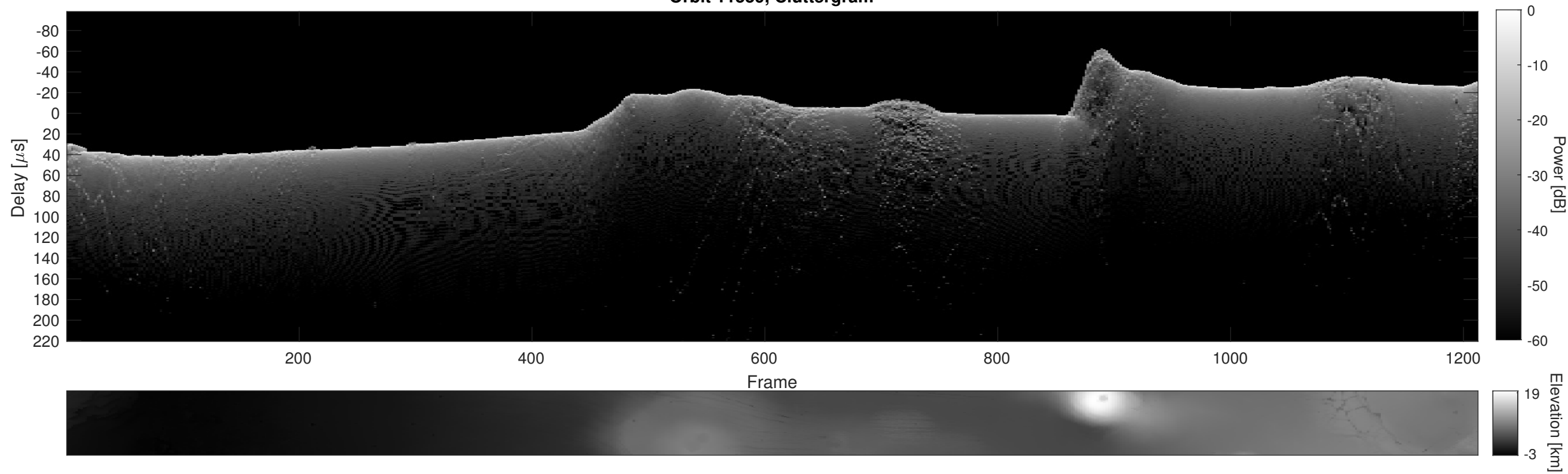
Orbit 11559, Cluttergram
