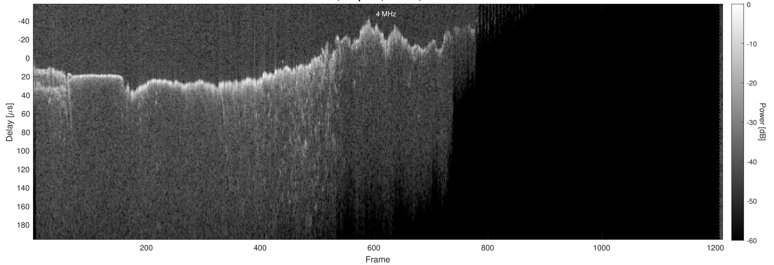
Orbit 11561, Chapman, Window, Channel 2
