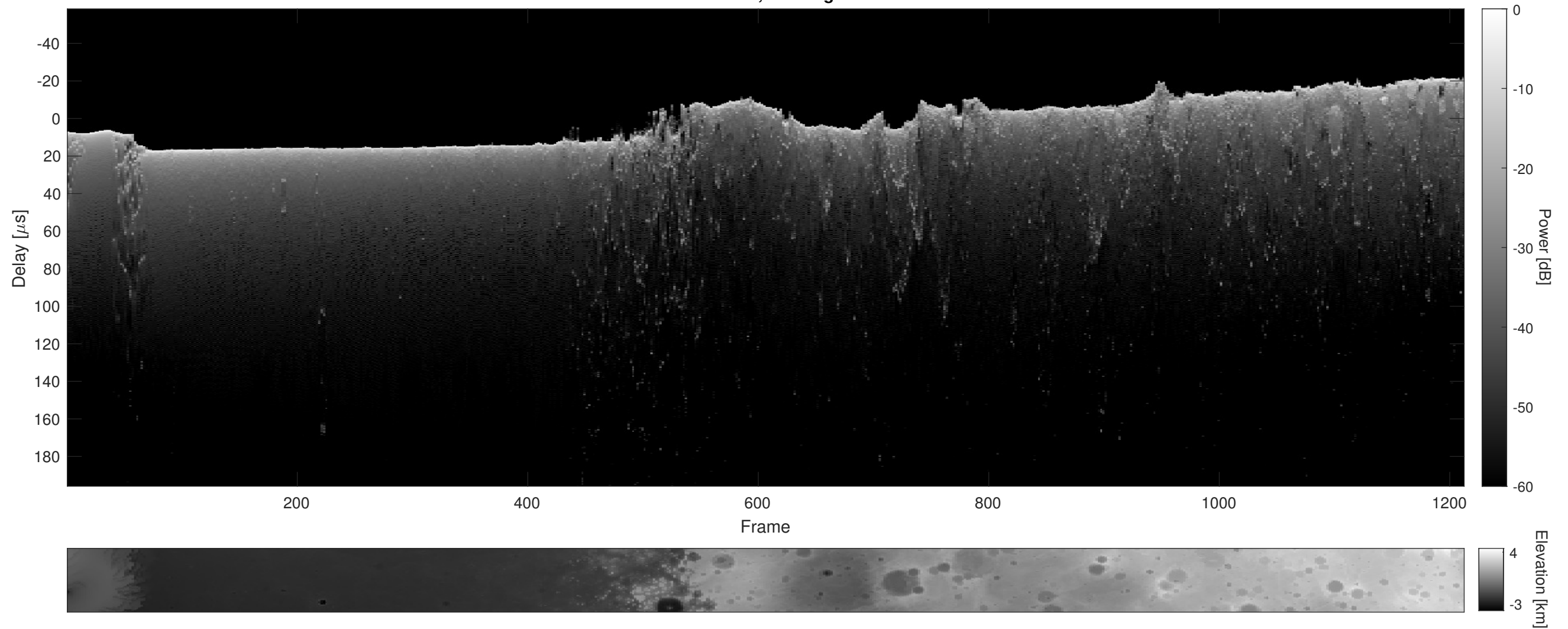
Orbit 11561, Cluttergram
