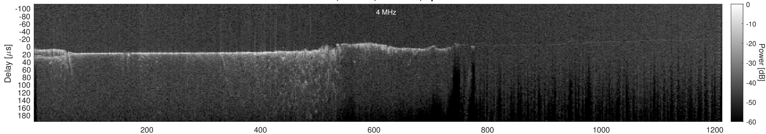
Orbit 11561, Cluttergram
