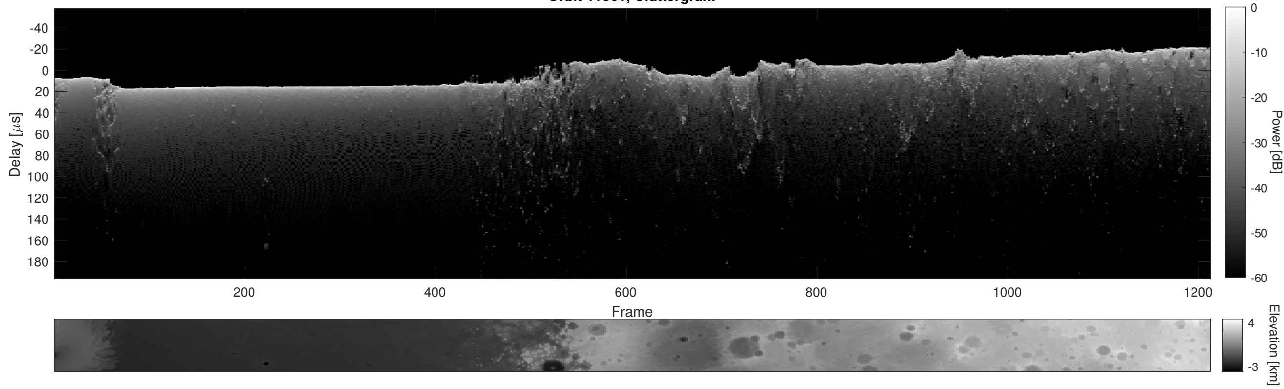
Orbit 11561, Cluttergram
