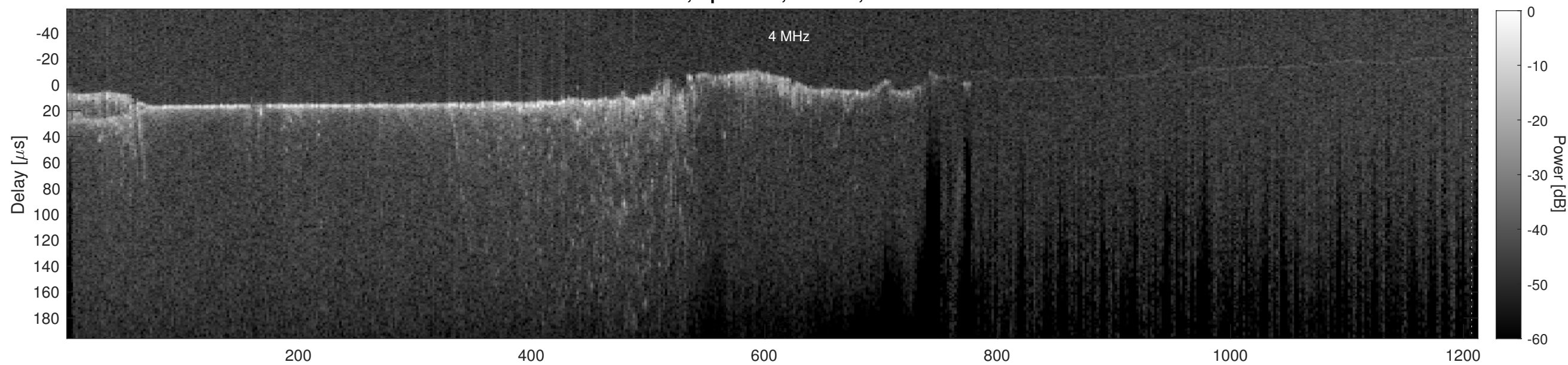
Orbit 11561, Cluttergram
