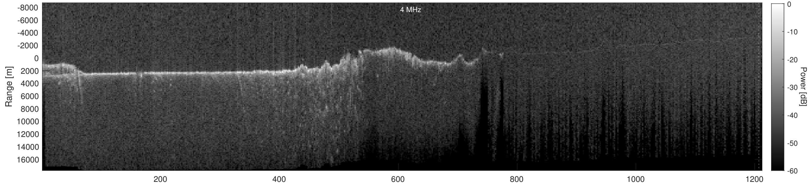
Orbit 11561, Depth-Corrected Cluttergram
