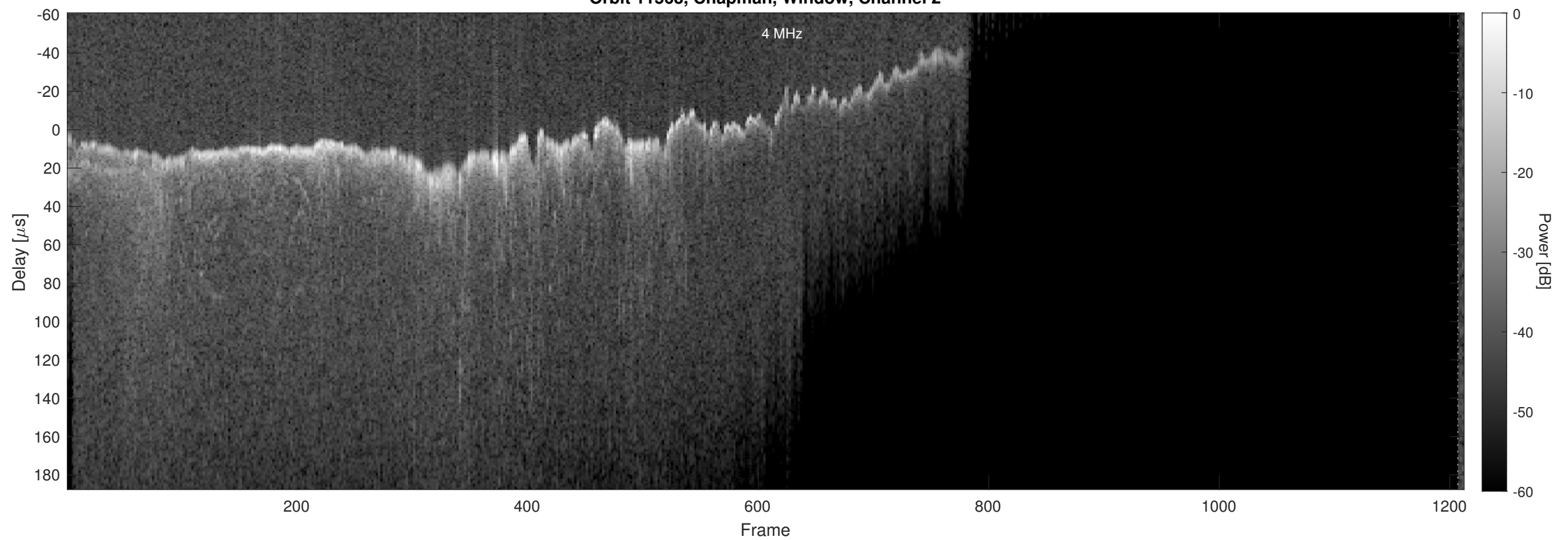
Orbit 11563, Chapman, Window, Channel 2
