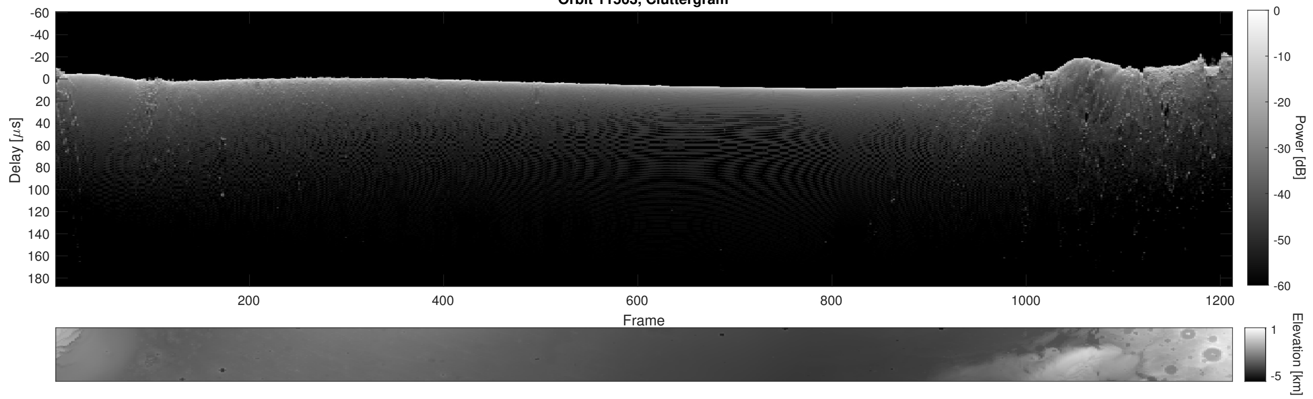
Orbit 11563, Cluttergram
