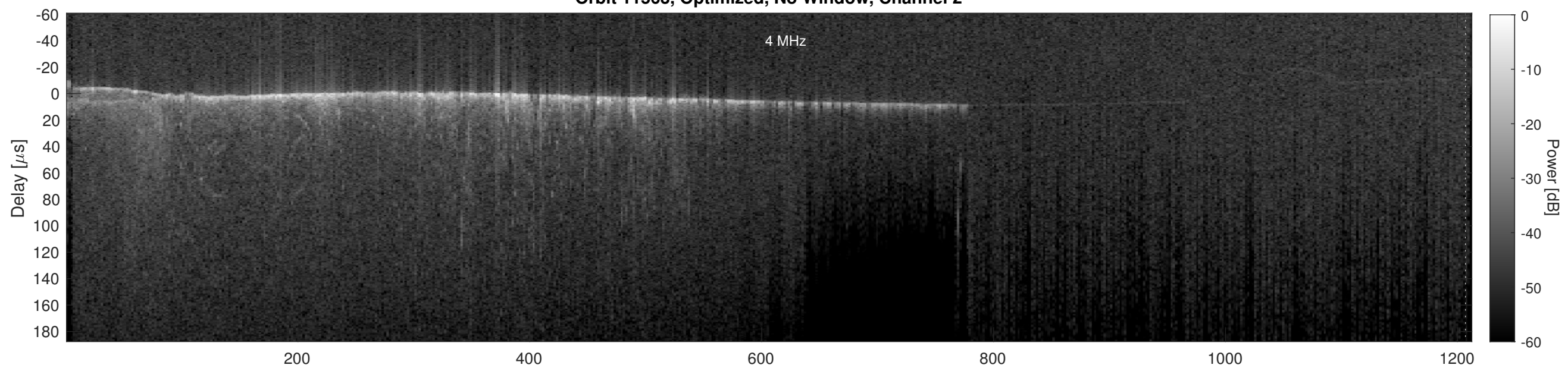
Orbit 11563, Cluttergram
