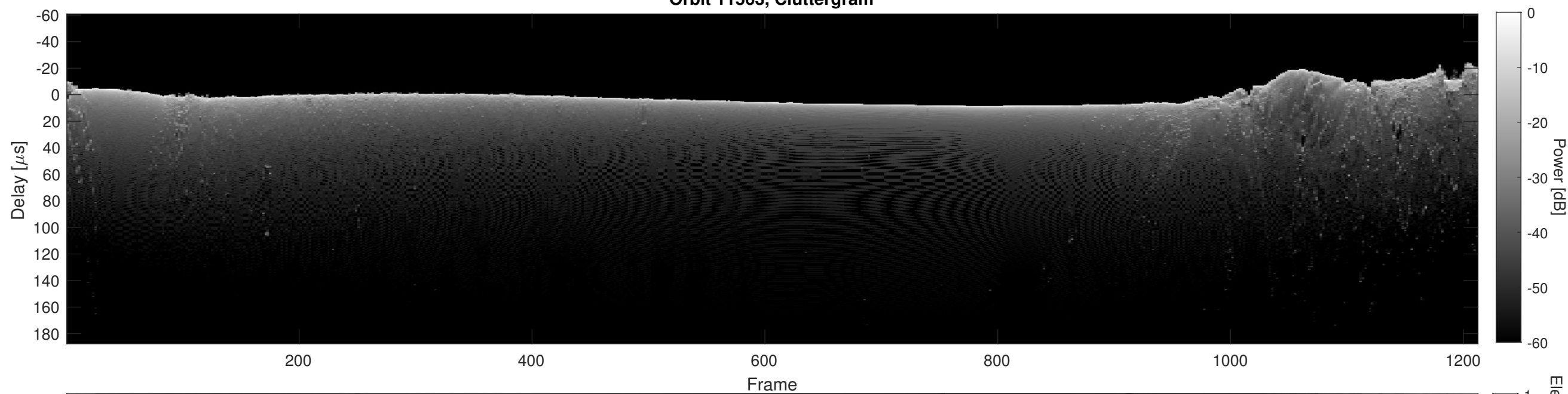
Orbit 11563, Cluttergram
