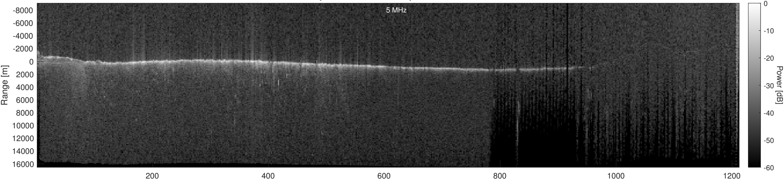
Orbit 11563, Optimized, Window, Depth-Corrected, Channel 2
