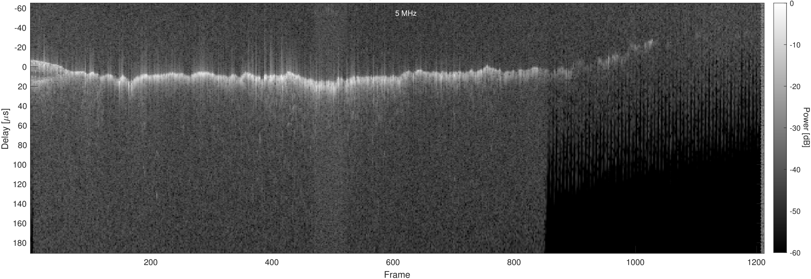
Orbit 11564, Chapman, No Window, Channel 2
