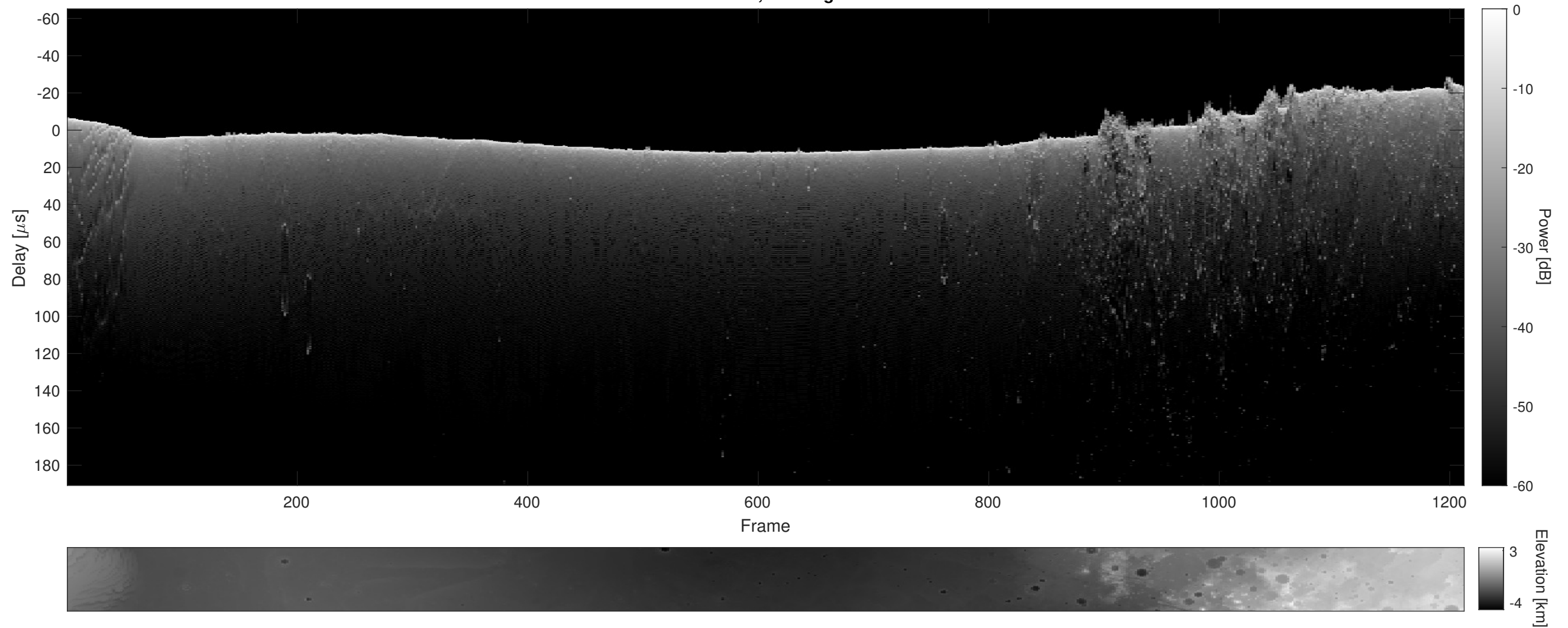
Orbit 11564, Cluttergram
