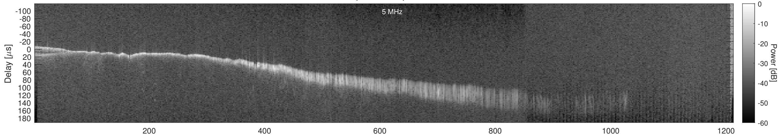
Orbit 11564, Window, Channel 1, Chapman
