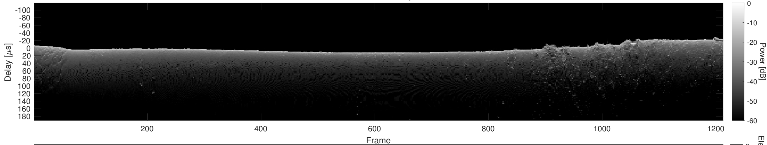
Orbit 11564, Cluttergram
