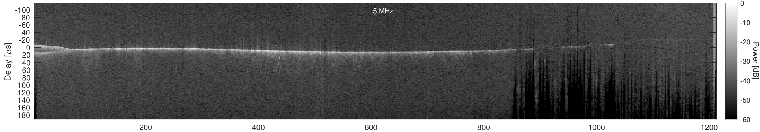
Orbit 11564, Cluttergram
