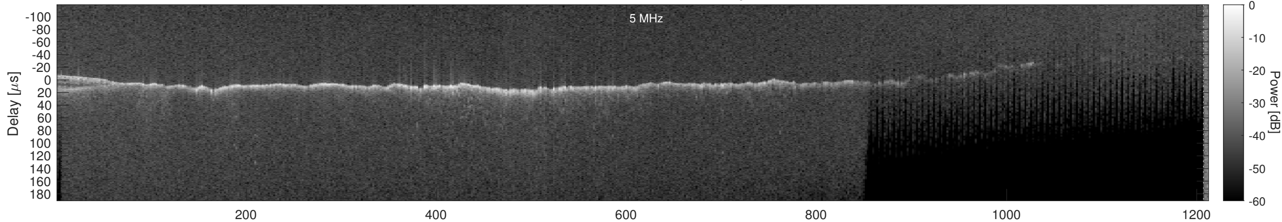
Orbit 11564, Window, Channel 1, Optimized
