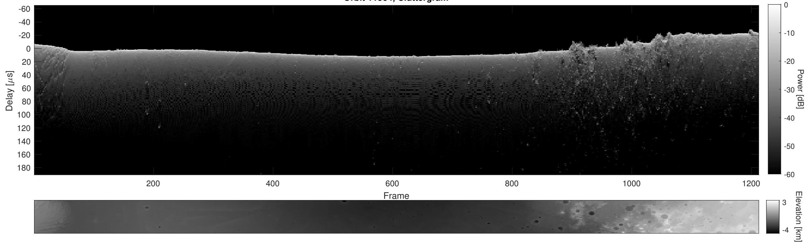
Orbit 11564, Cluttergram
