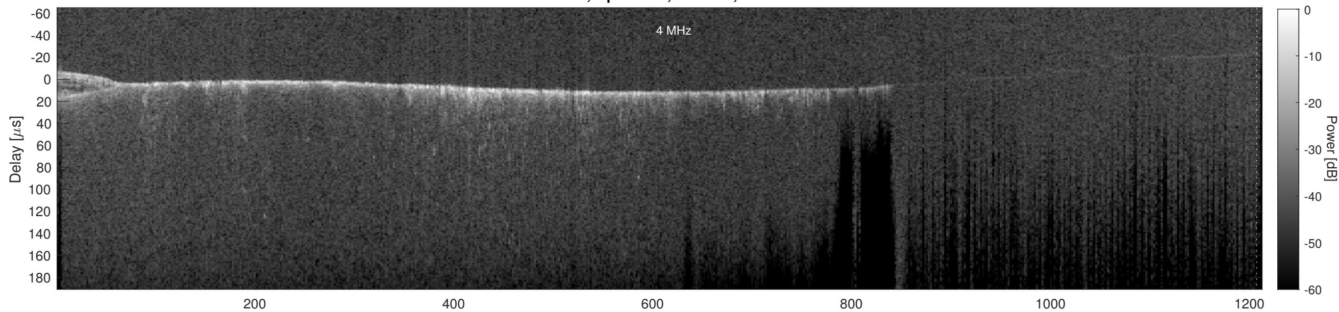
Orbit 11564, Cluttergram
