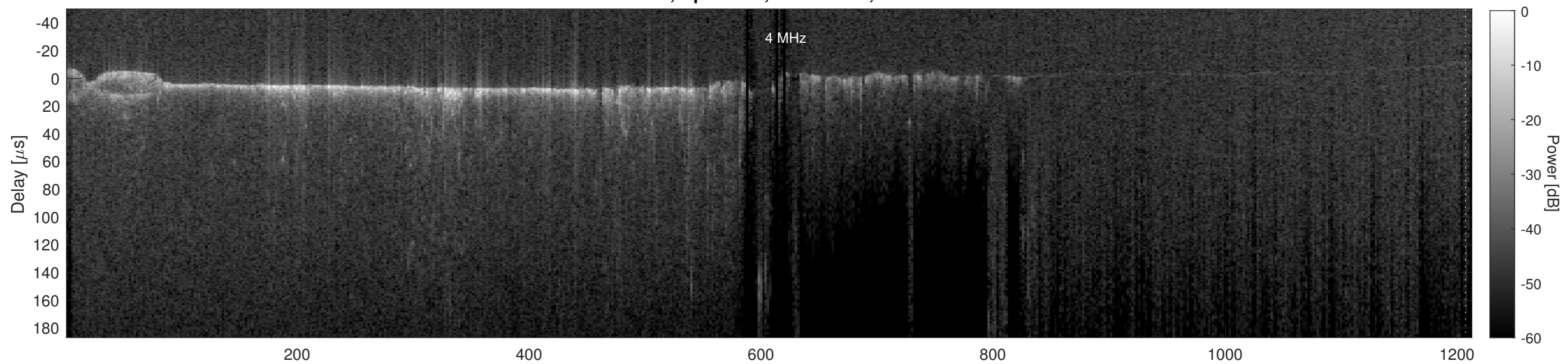
Orbit 11565, Cluttergram
