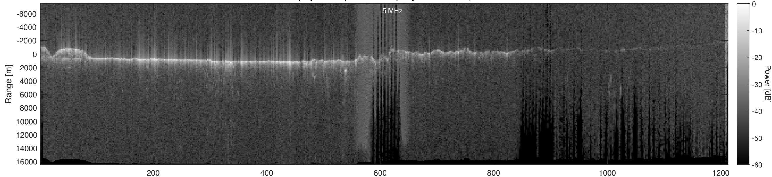
Orbit 11565, Optimized, No Window, Depth-Corrected, Channel 2
