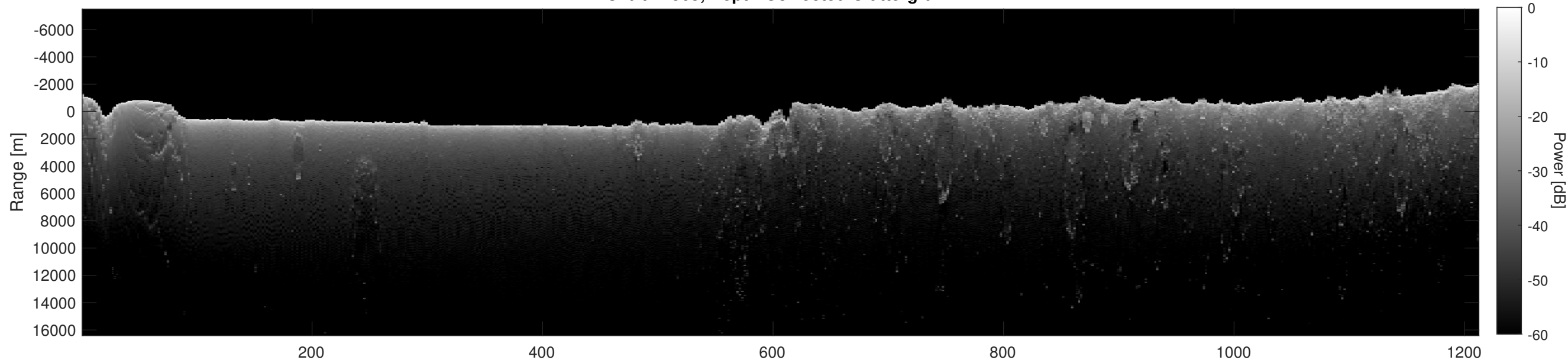
Orbit 11565, Depth-Corrected Cluttergram
