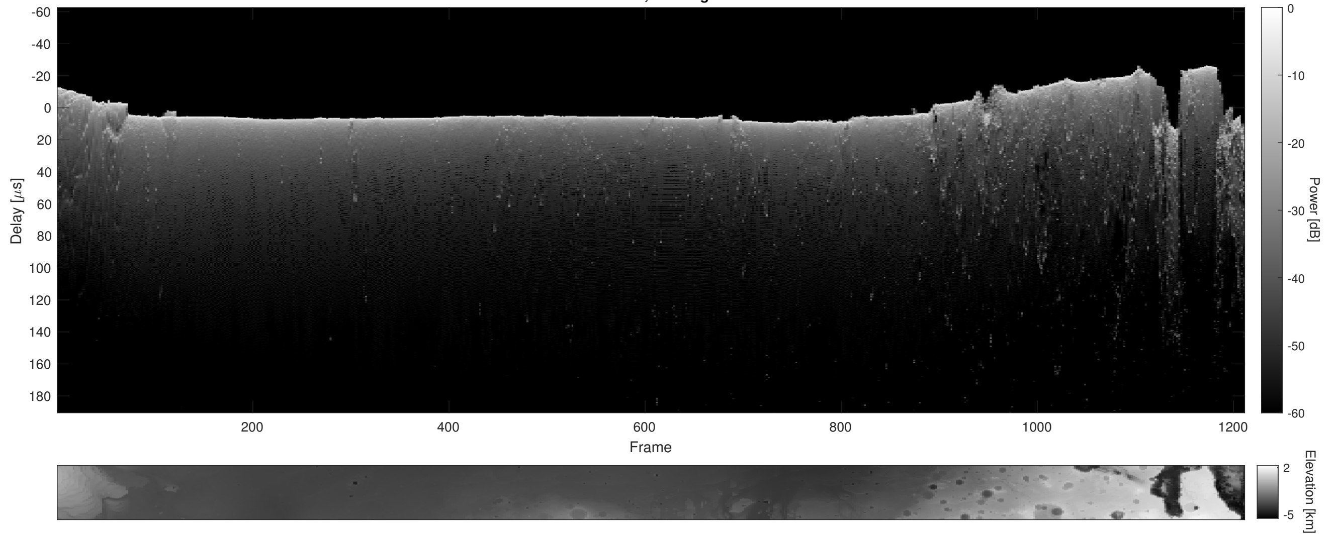
Orbit 11569, Cluttergram
