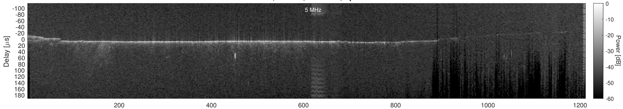
Orbit 11569, Cluttergram
