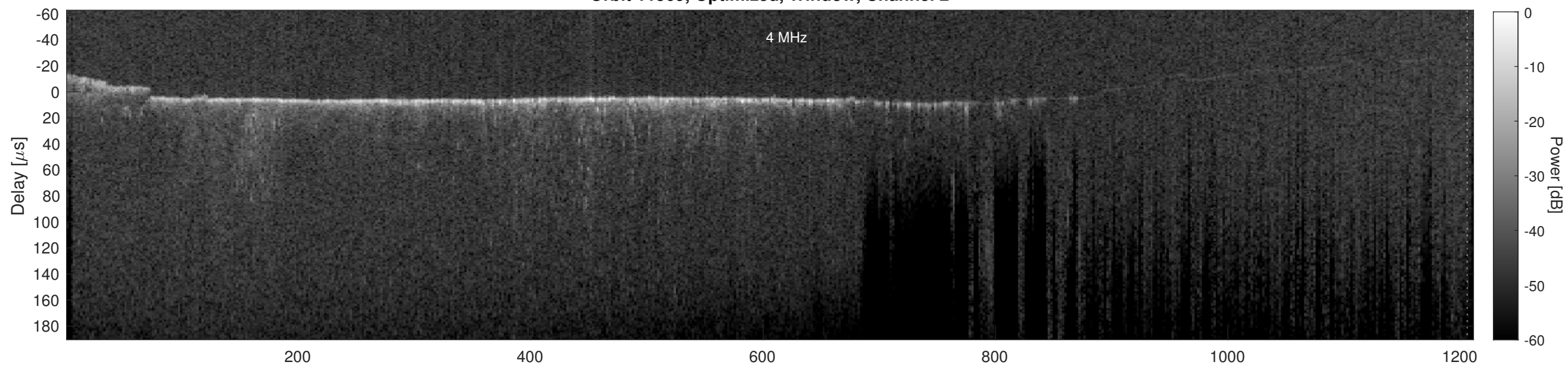
Orbit 11569, Cluttergram
