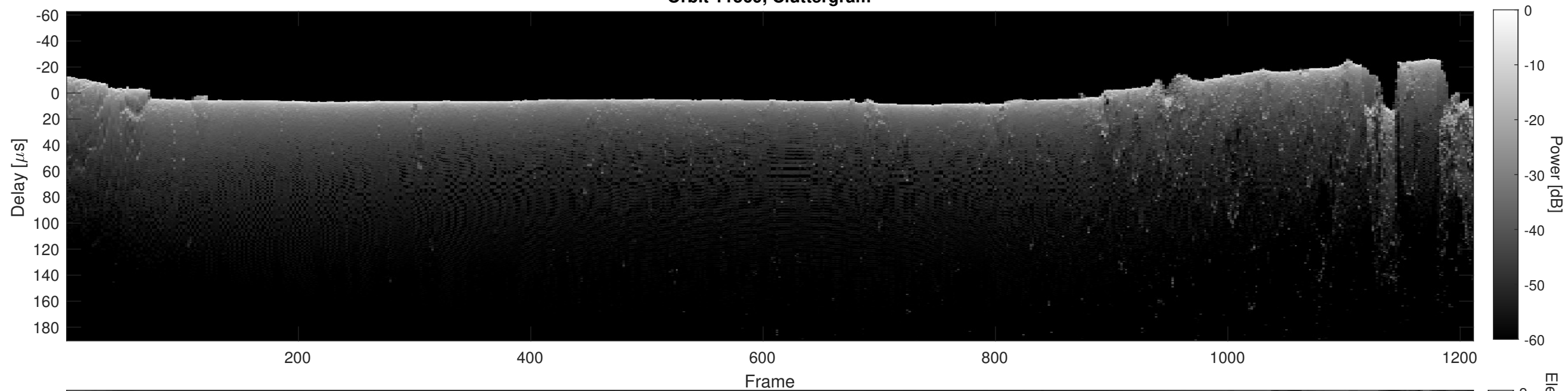
Orbit 11569, Cluttergram
