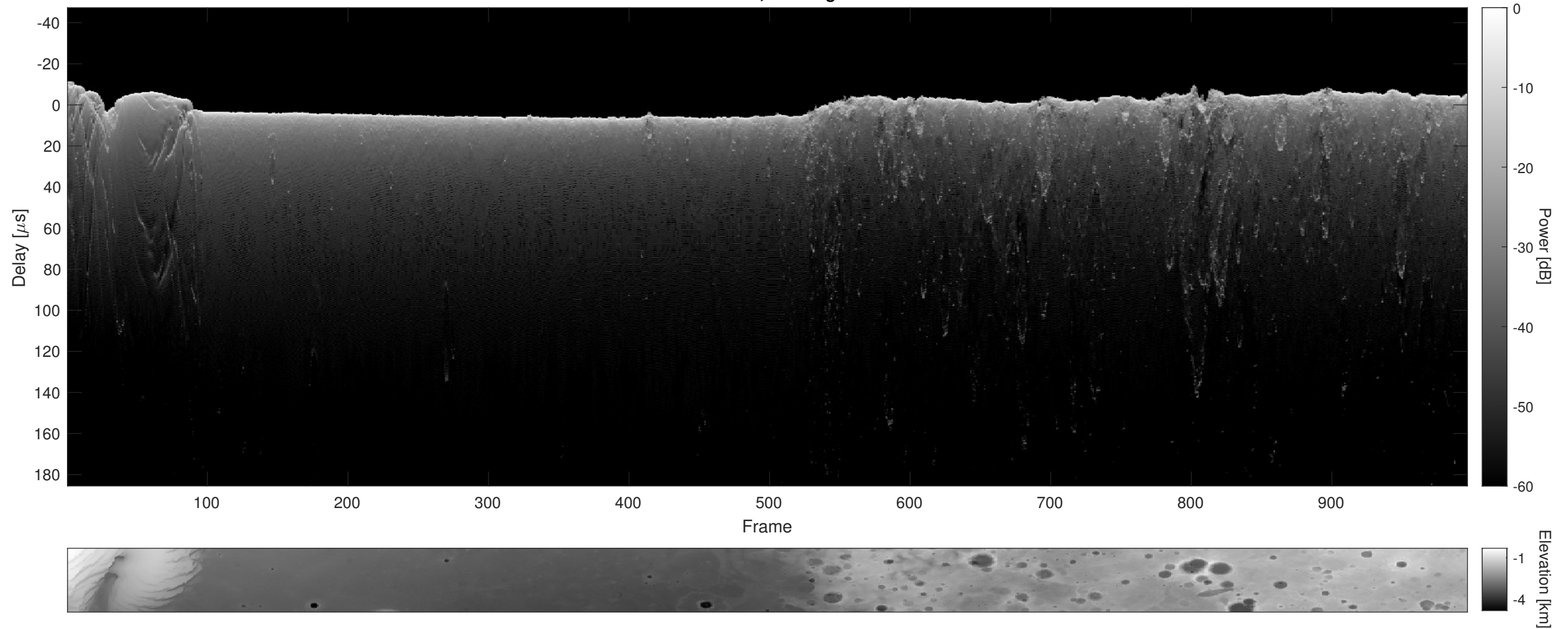
Orbit 11572, Cluttergram
