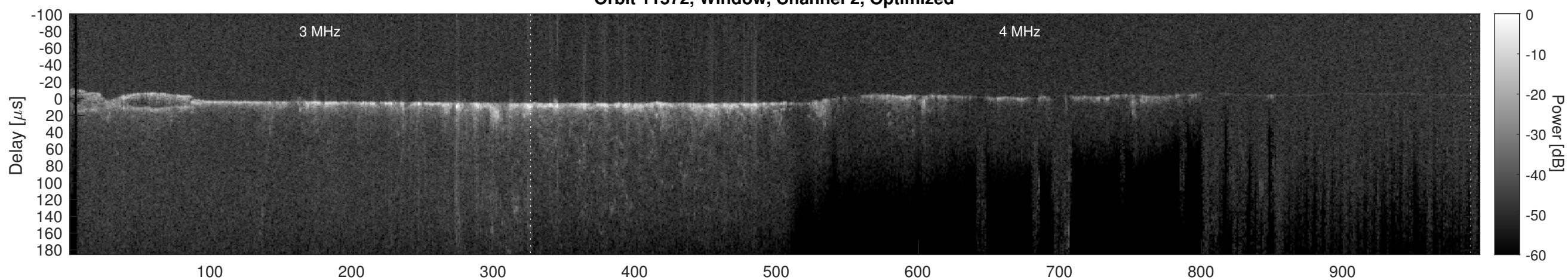
Orbit 11572, Cluttergram
