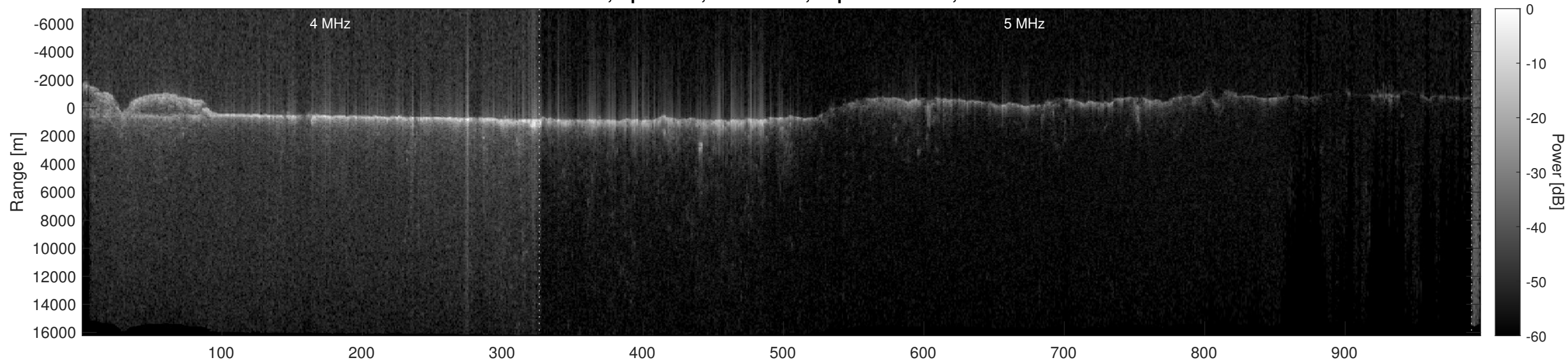
Orbit 11572, Optimized, No Window, Depth-Corrected, Channel 2
