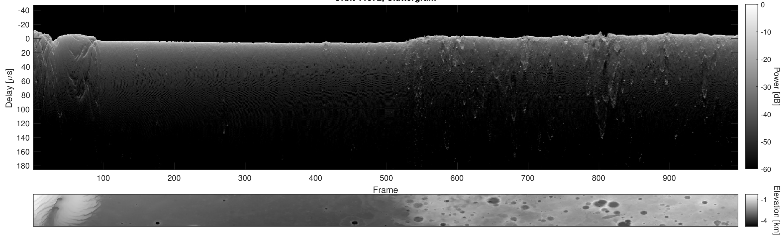
Orbit 11572, Cluttergram
