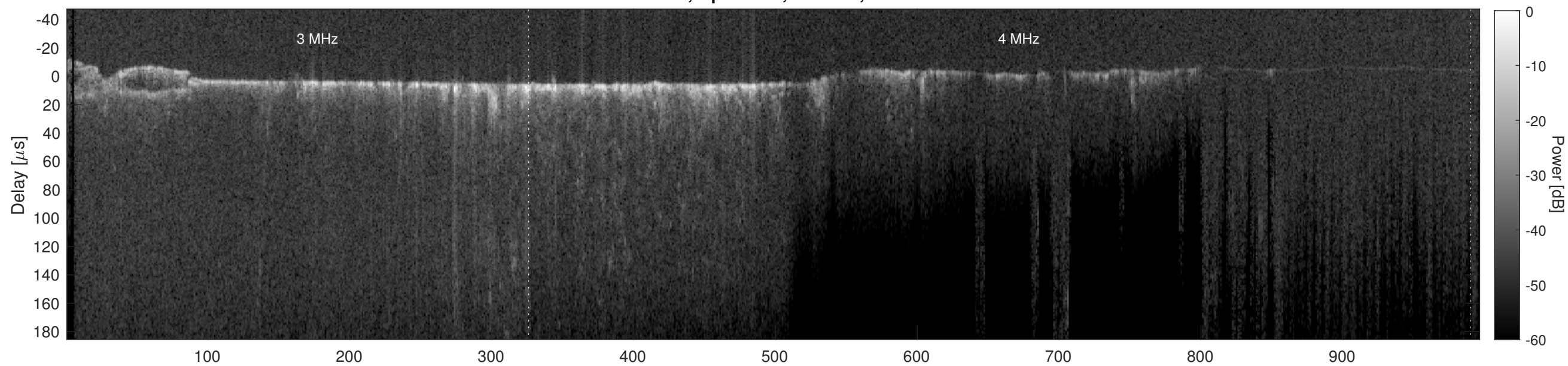
Orbit 11572, Cluttergram
