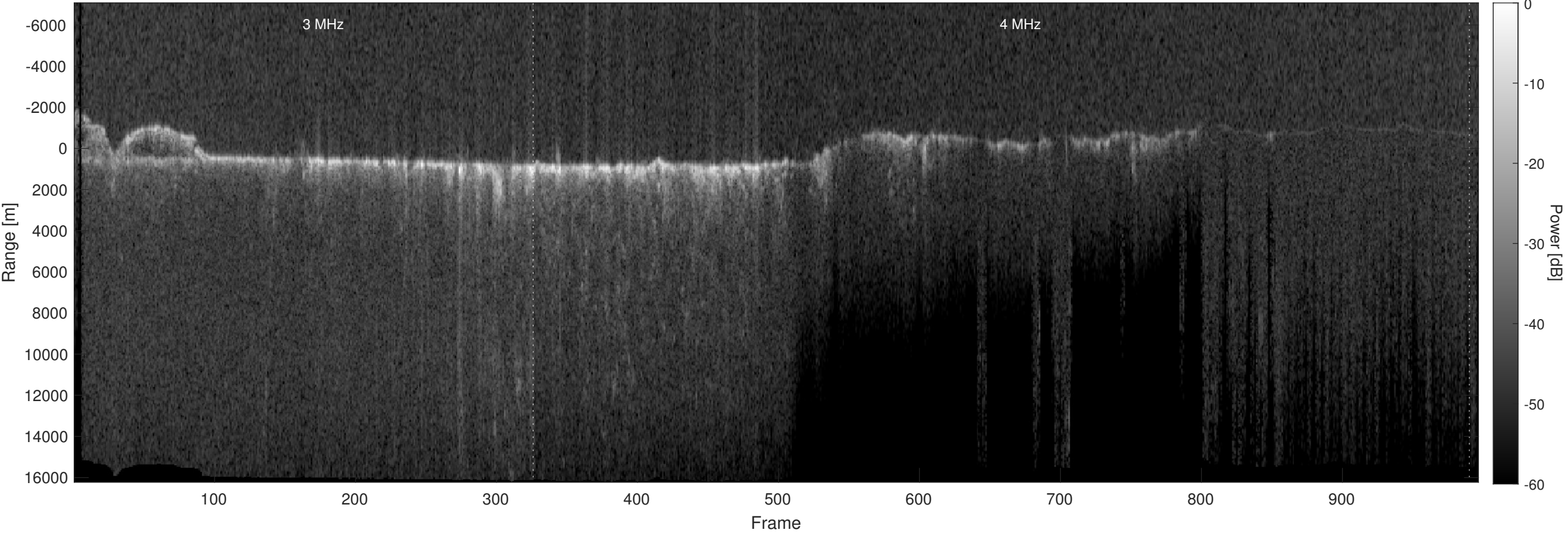
Orbit 11572, Optimized, Window, Depth-Corrected, Channel 2
