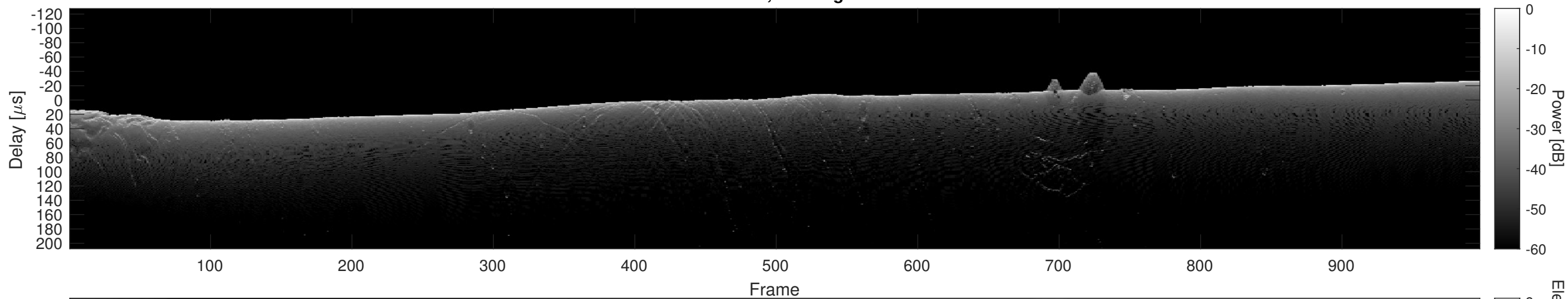
Orbit 11573, Cluttergram
