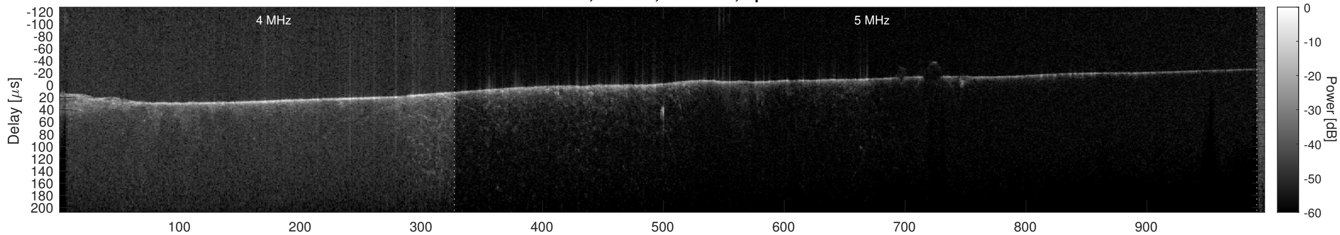
Orbit 11573, Cluttergram
