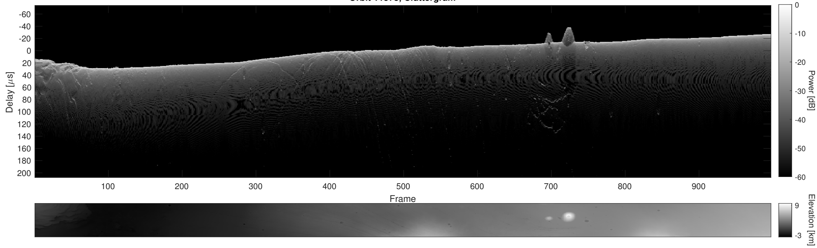
Orbit 11573, Cluttergram
