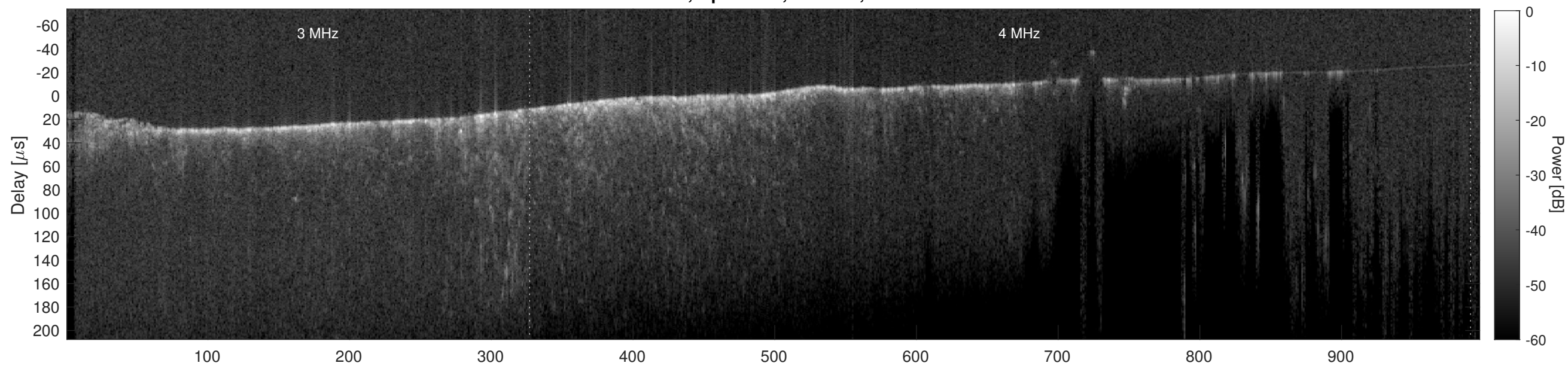
Orbit 11573, Cluttergram
