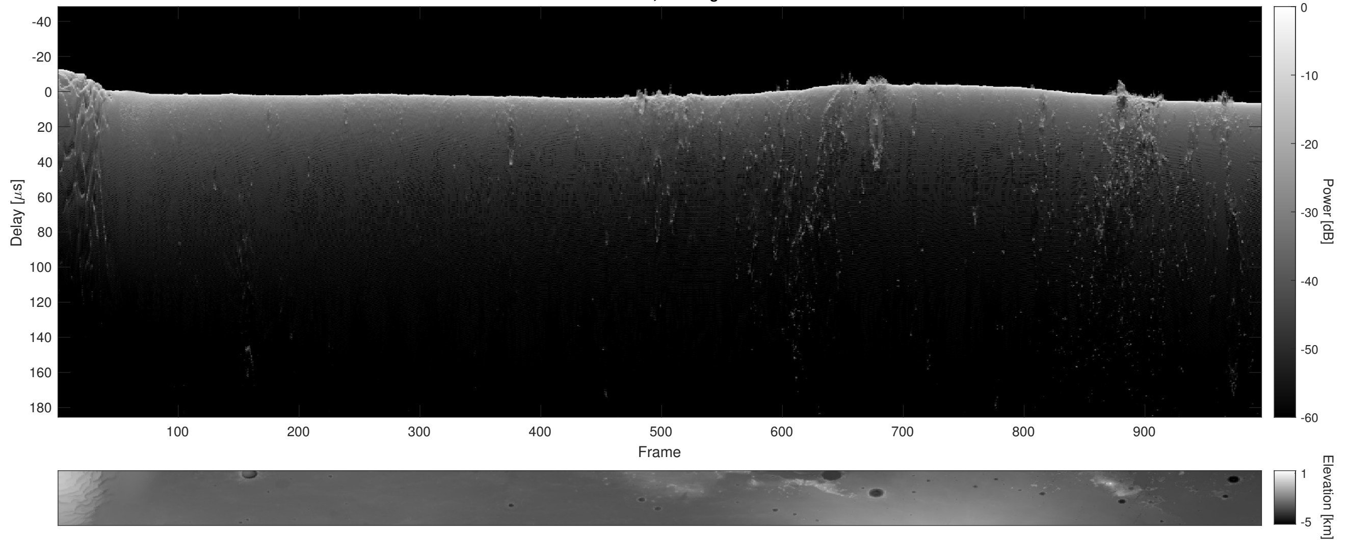
Orbit 11574, Cluttergram
