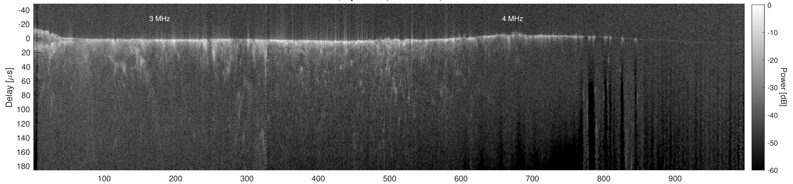
Orbit 11574, Cluttergram
