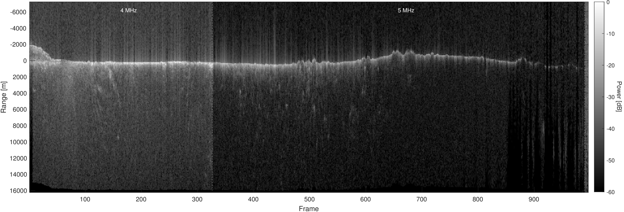
Orbit 11574, Optimized, No Window, Depth-Corrected, Channel 2
