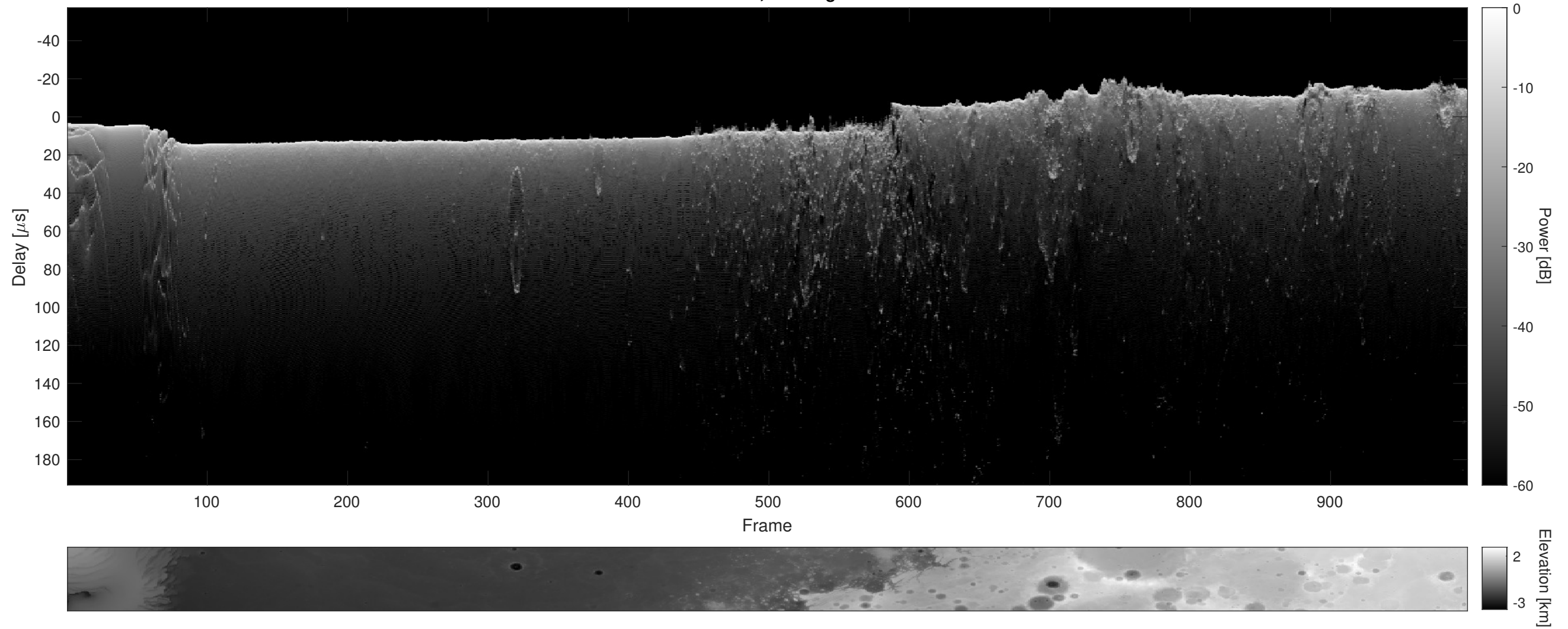
Orbit 11575, Cluttergram
