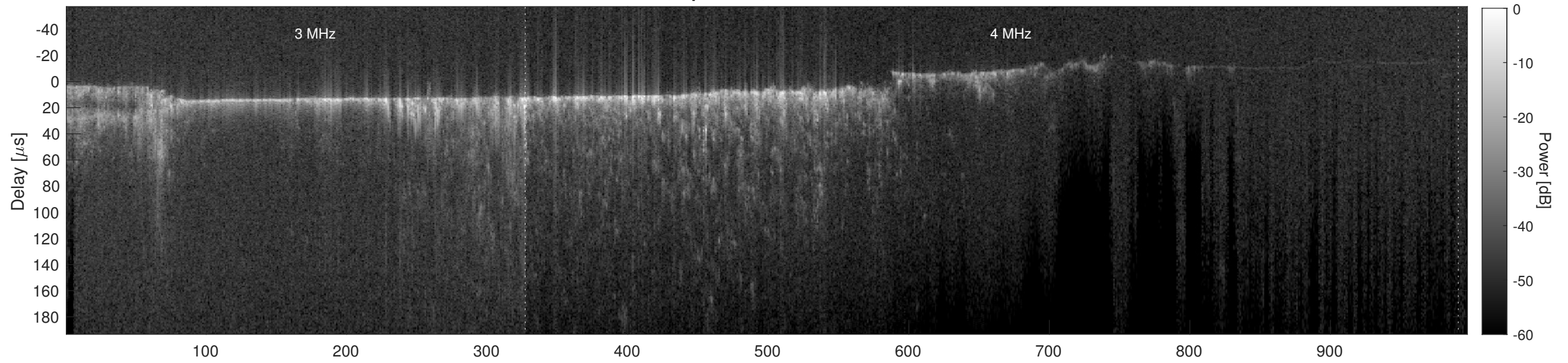
Orbit 11575, Cluttergram
