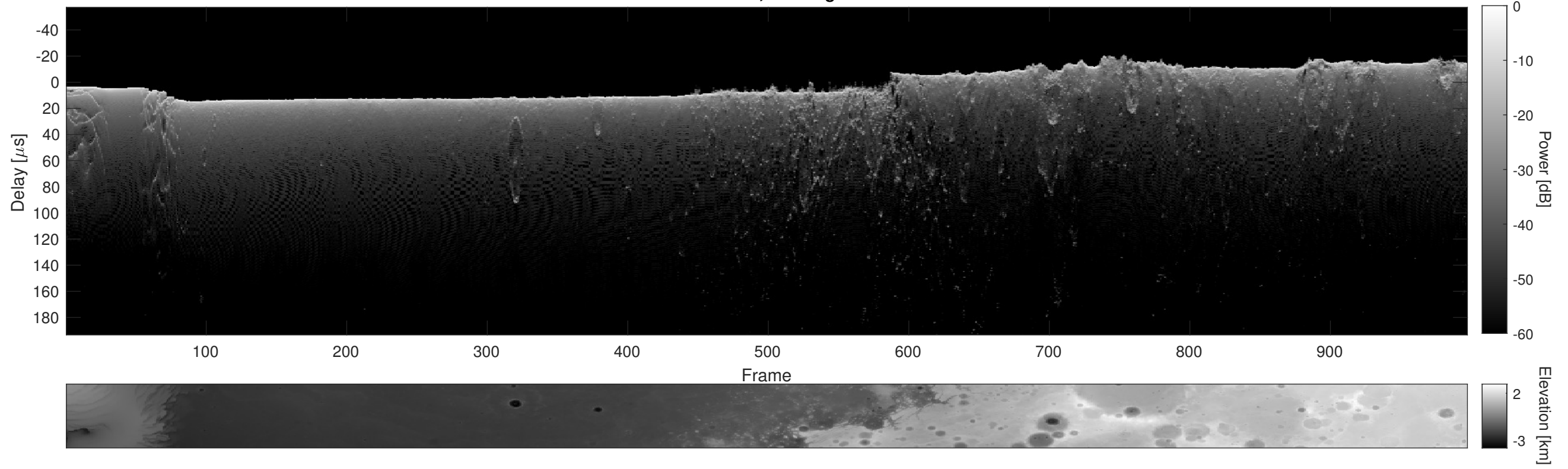
Orbit 11575, Cluttergram
