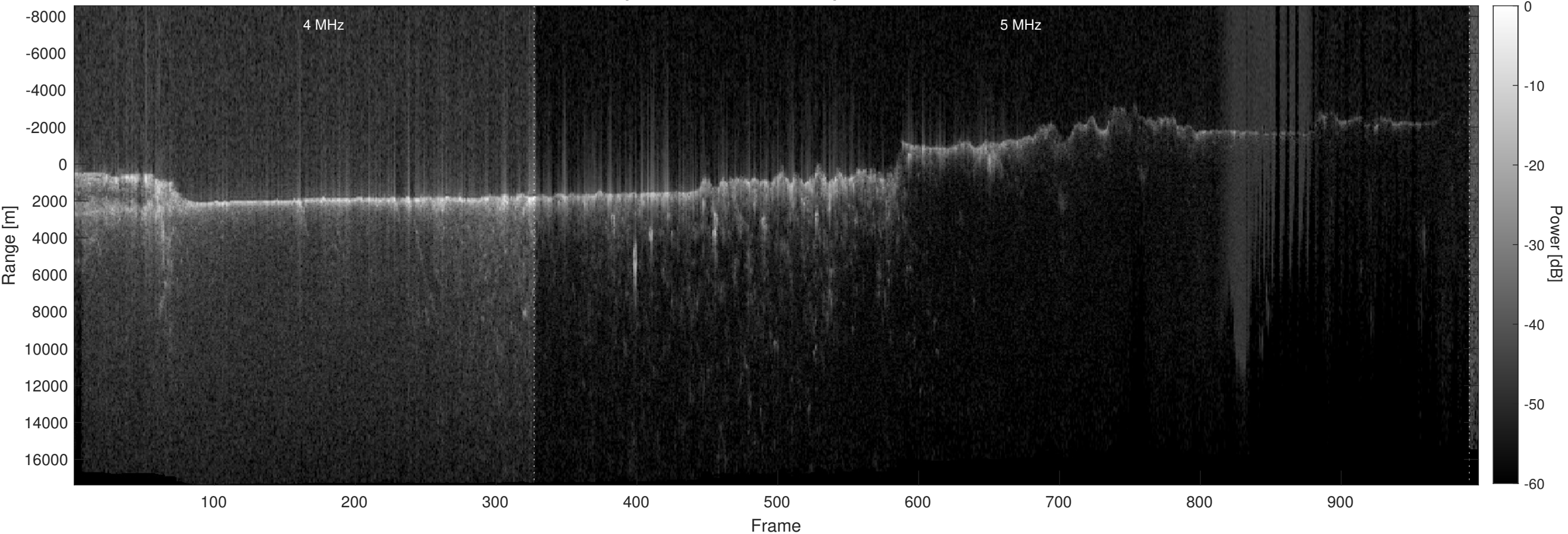
Orbit 11575, Optimized, No Window, Depth-Corrected, Channel 2
