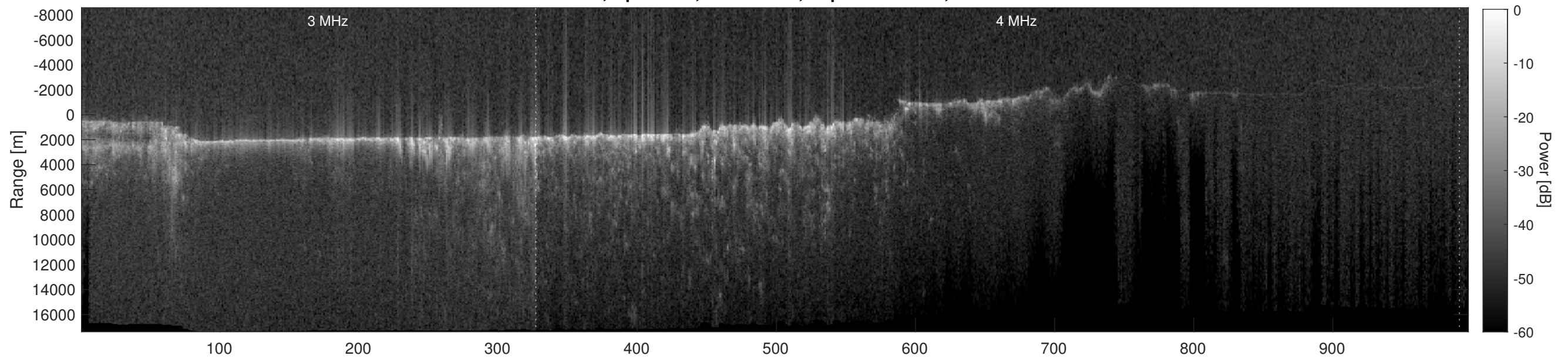
Orbit 11575, Depth-Corrected Cluttergram
