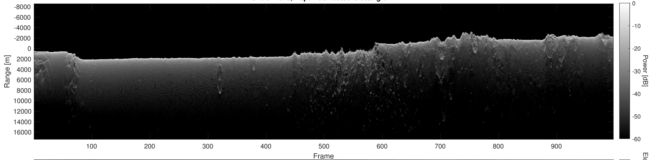
Orbit 11575, Depth-Corrected Cluttergram
