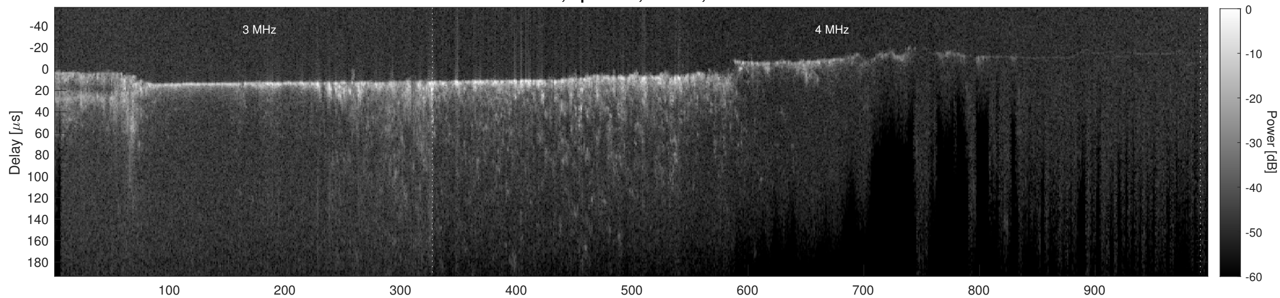
Orbit 11575, Cluttergram
