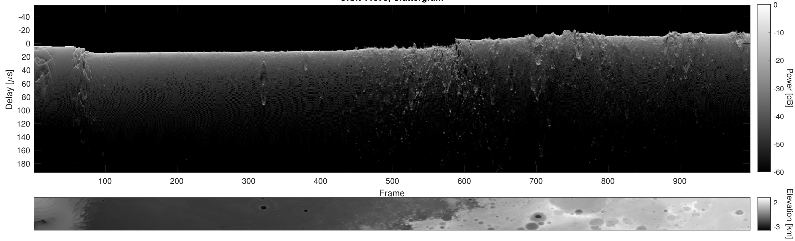
Orbit 11575, Cluttergram
