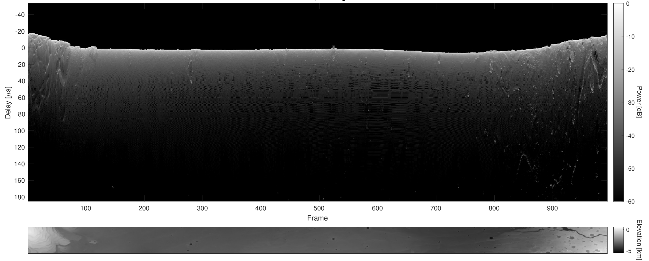
Orbit 11576, Cluttergram
