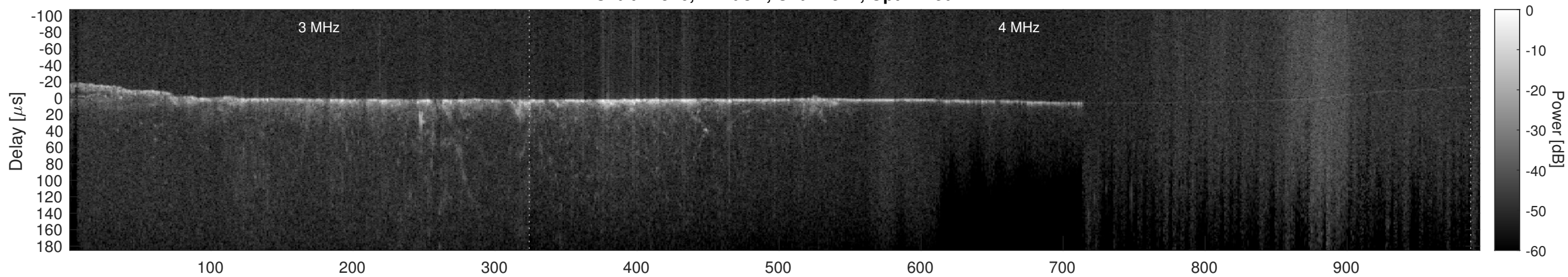
Orbit 11576, Cluttergram
