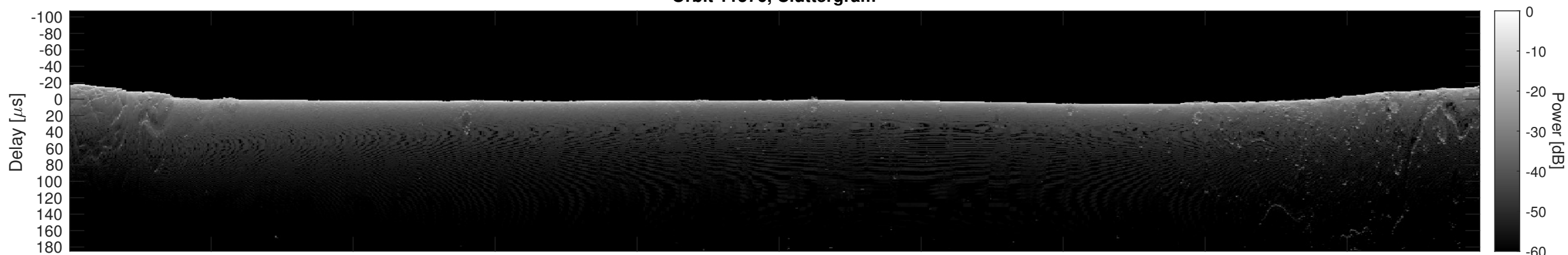
Orbit 11576, Cluttergram
