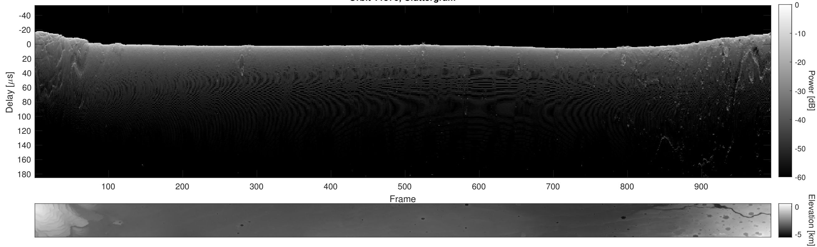
Orbit 11576, Cluttergram
