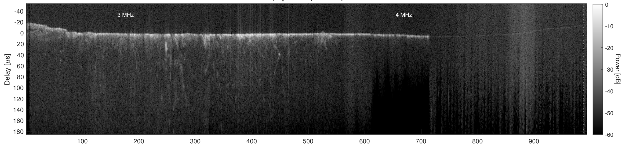
Orbit 11576, Cluttergram
