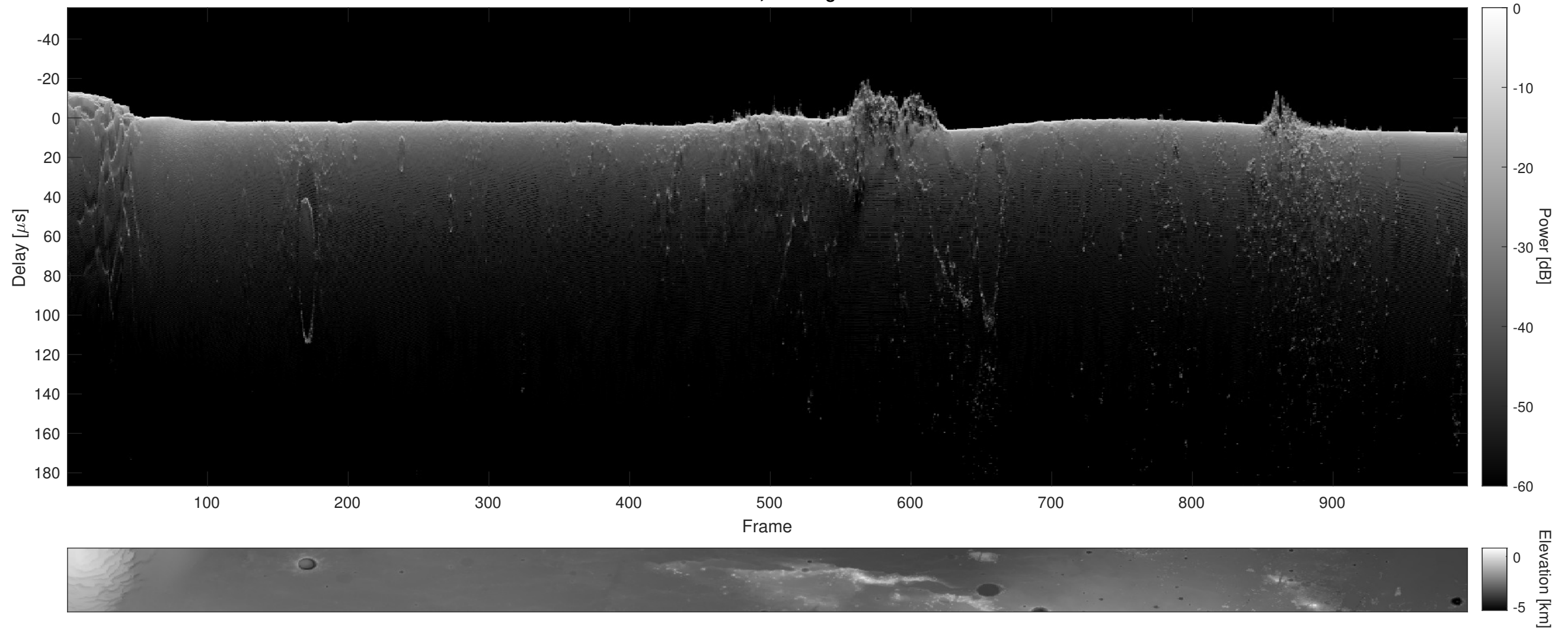
Orbit 11581, Cluttergram
