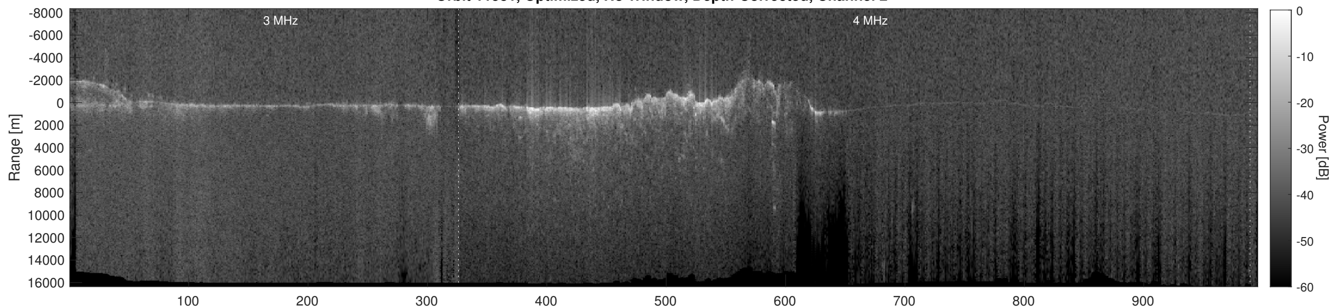
Orbit 11581, Depth-Corrected Cluttergram
