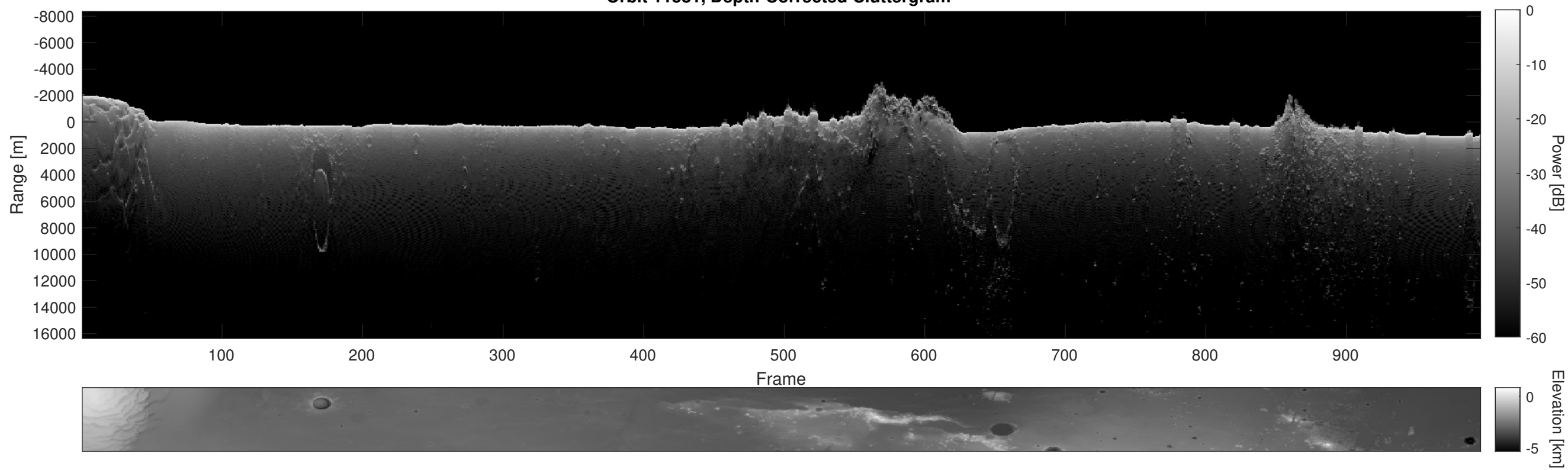
Orbit 11581, Depth-Corrected Cluttergram
