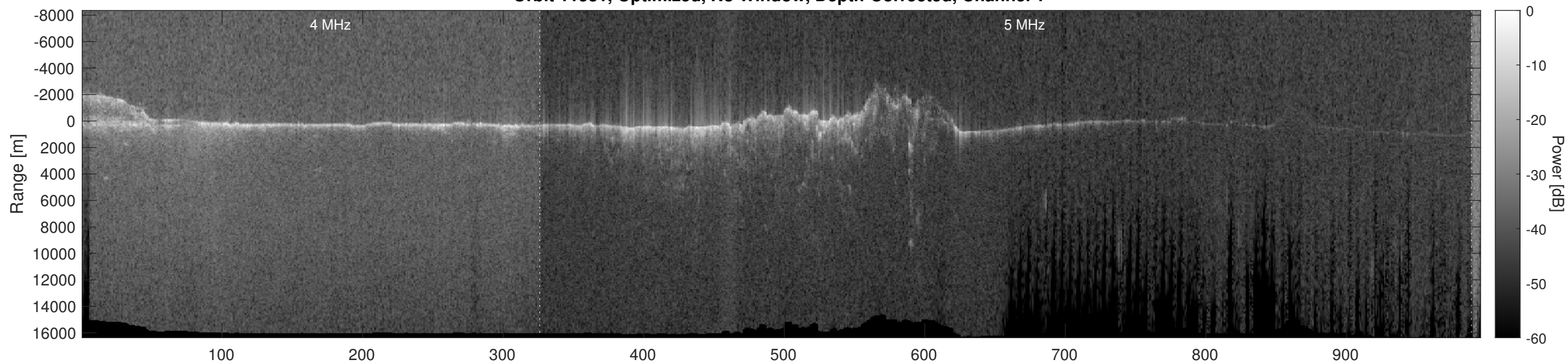
Orbit 11581, Optimized, No Window, Depth-Corrected, Channel 2
