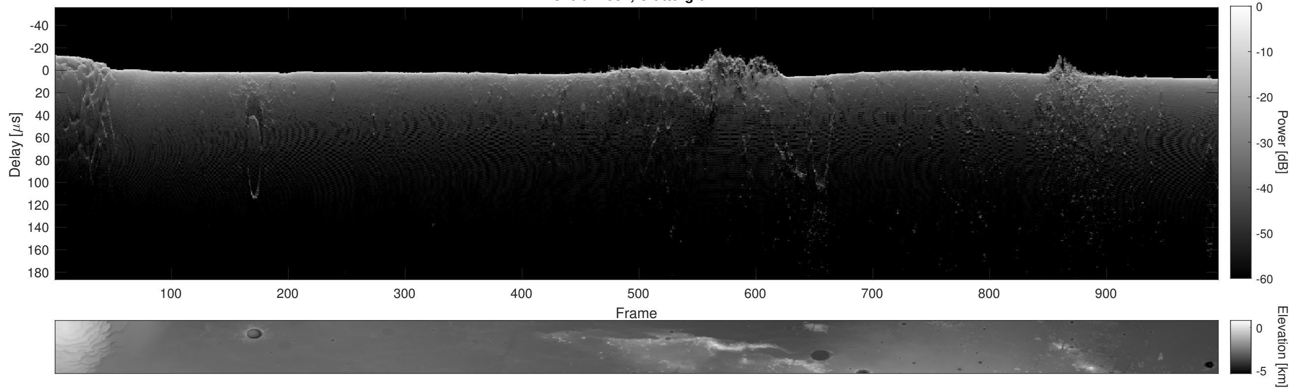
Orbit 11581, Cluttergram
