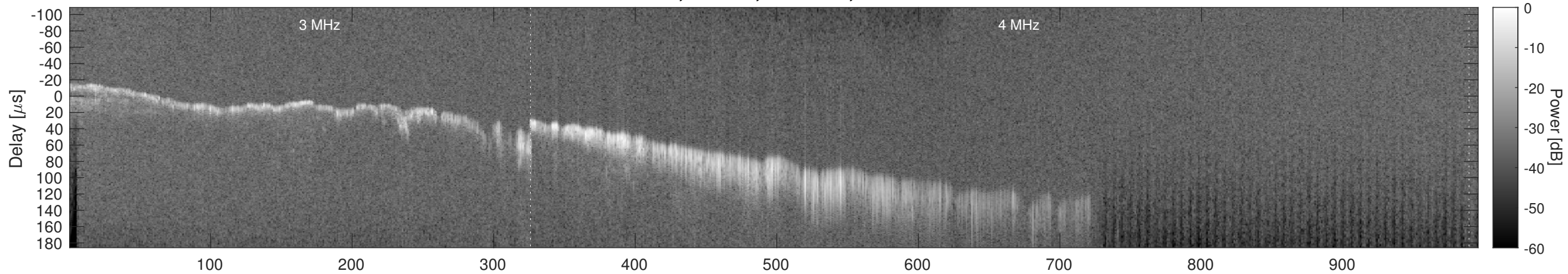
Orbit 11583, Window, Channel 2, Chapman
