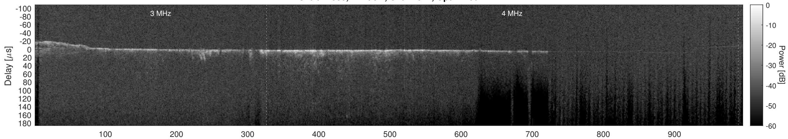
Orbit 11583, Cluttergram
