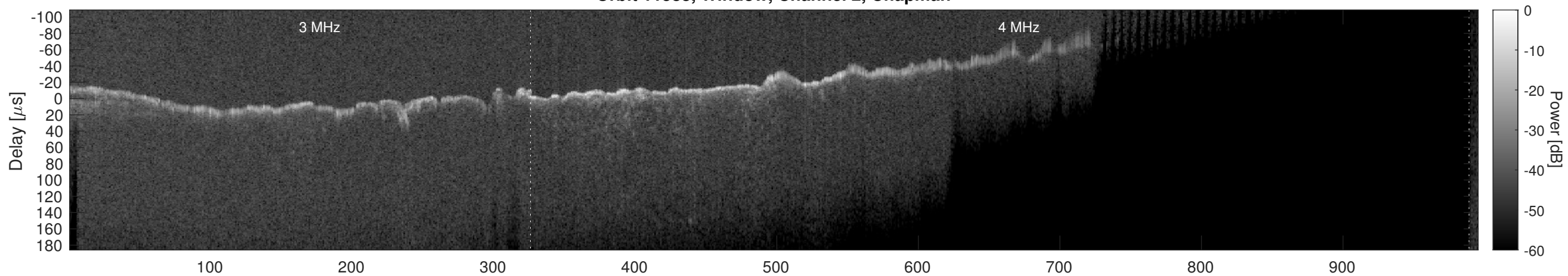
Orbit 11583, Window, Channel 2, Optimized
