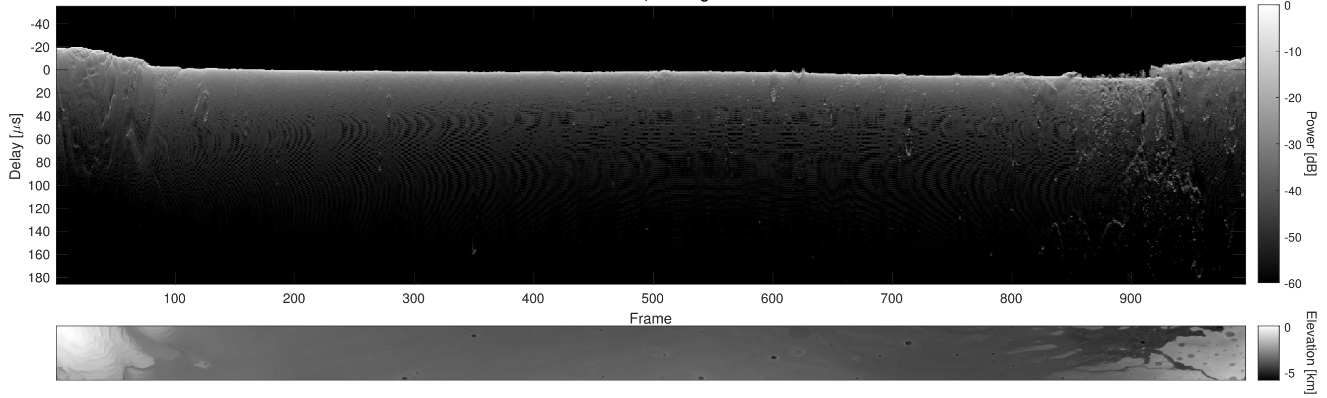
Orbit 11583, Cluttergram
