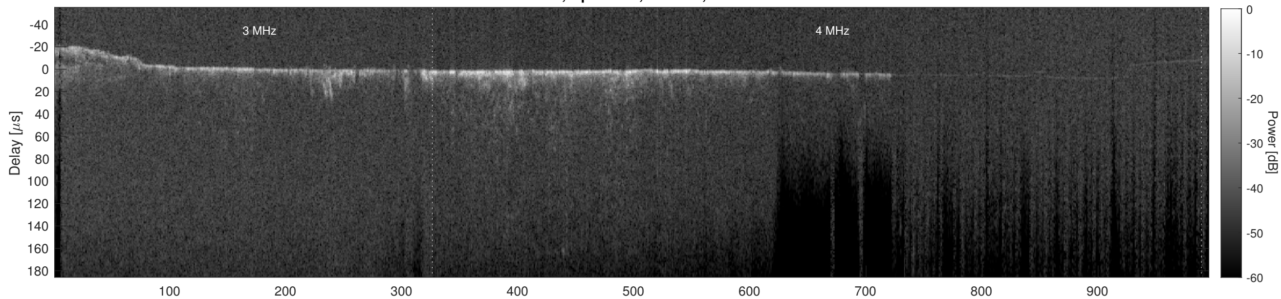
Orbit 11583, Cluttergram
