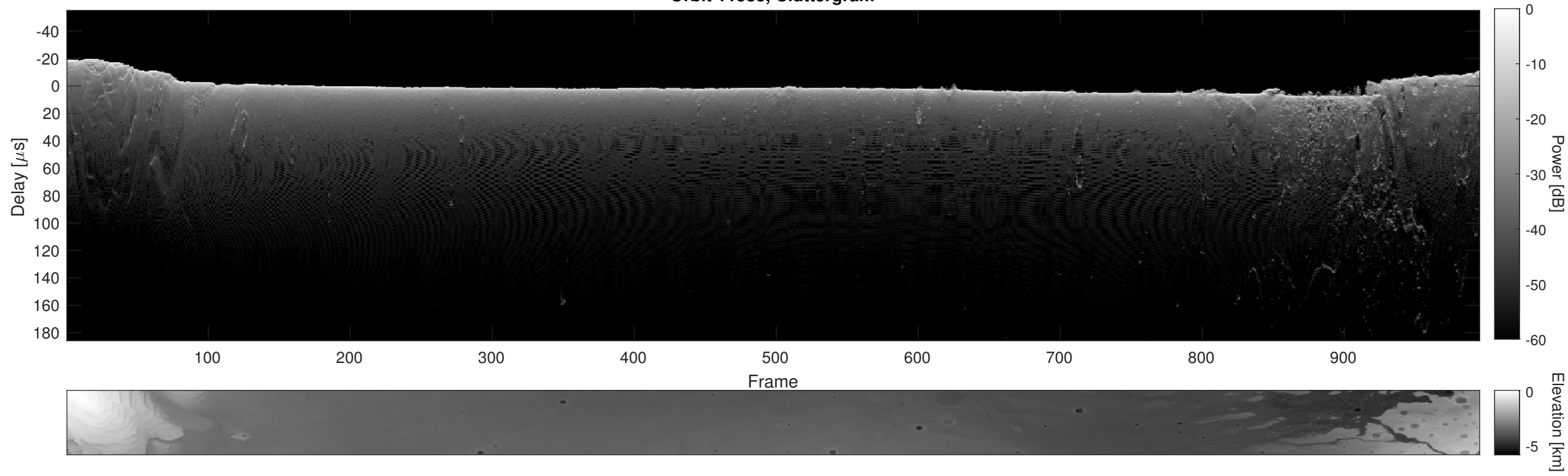
Orbit 11583, Cluttergram
