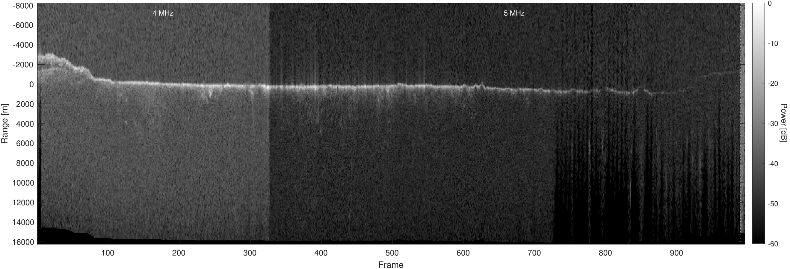
Orbit 11583, Optimized, Window, Depth-Corrected, Channel 2
