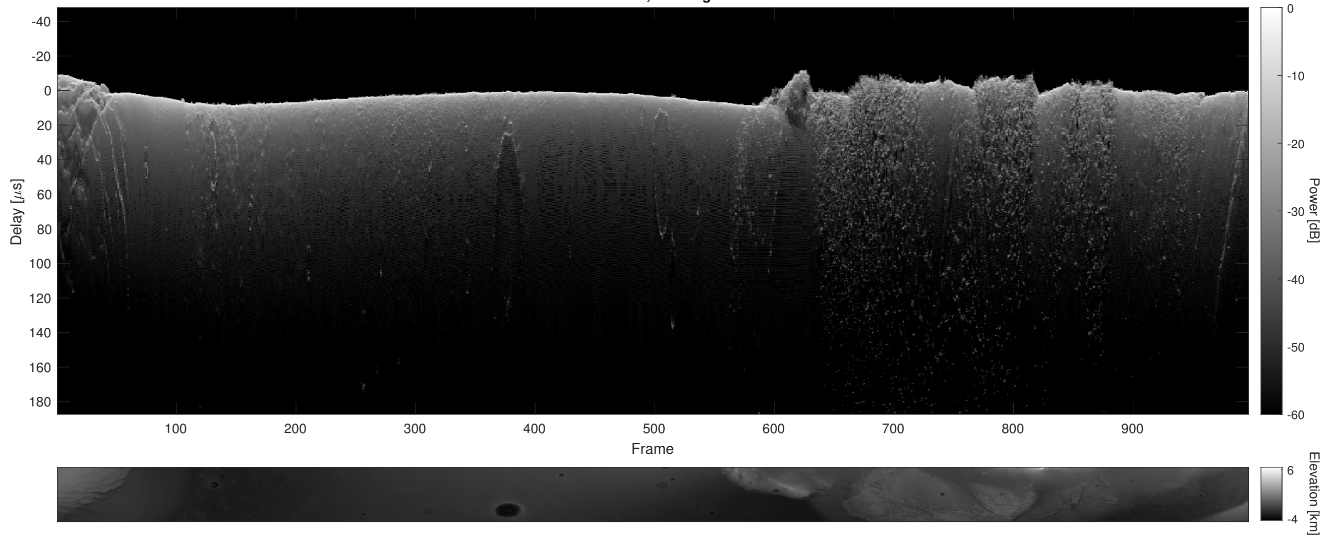
Orbit 11584, Cluttergram
