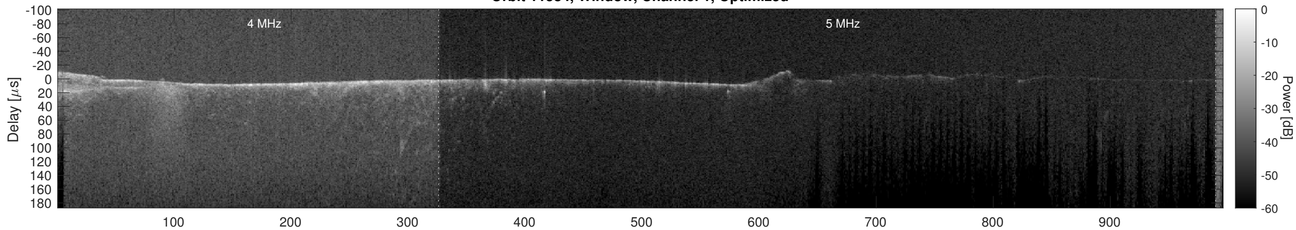
Orbit 11584, Cluttergram
