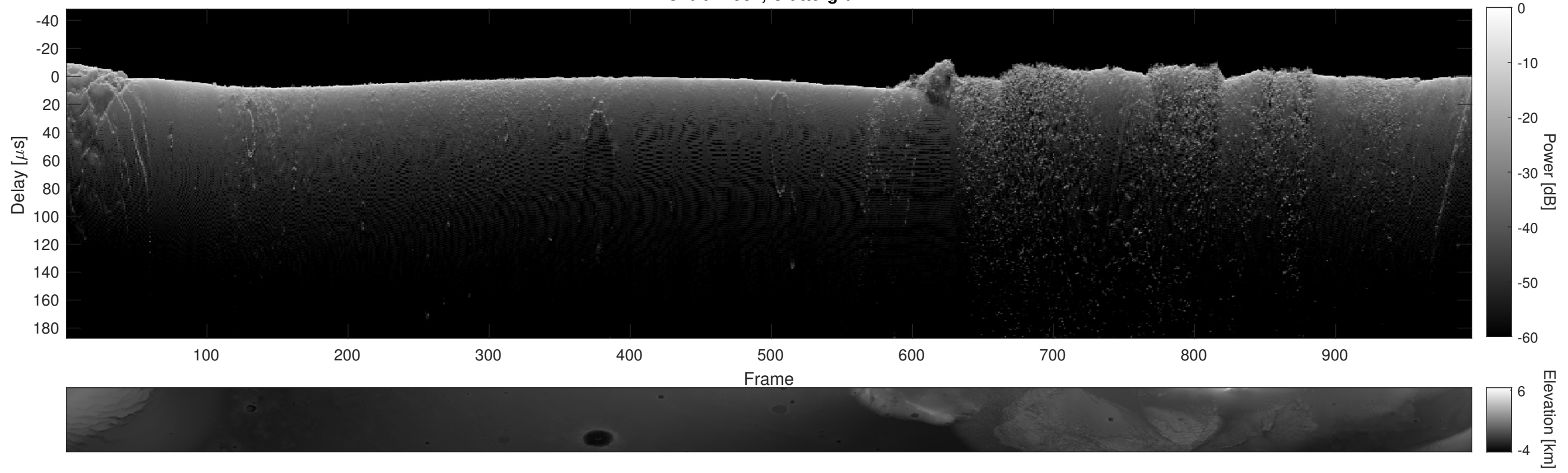
Orbit 11584, Cluttergram
