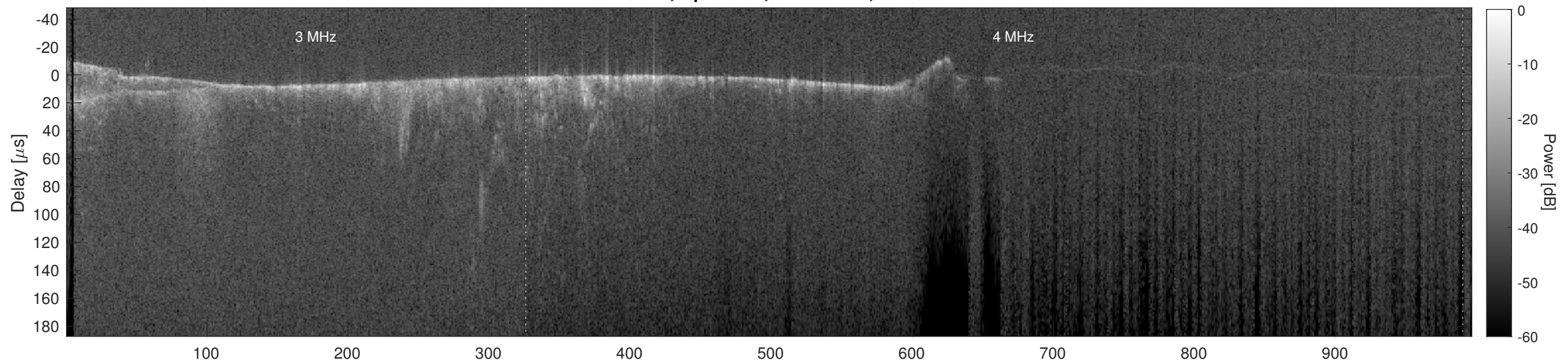
Orbit 11584, Cluttergram
